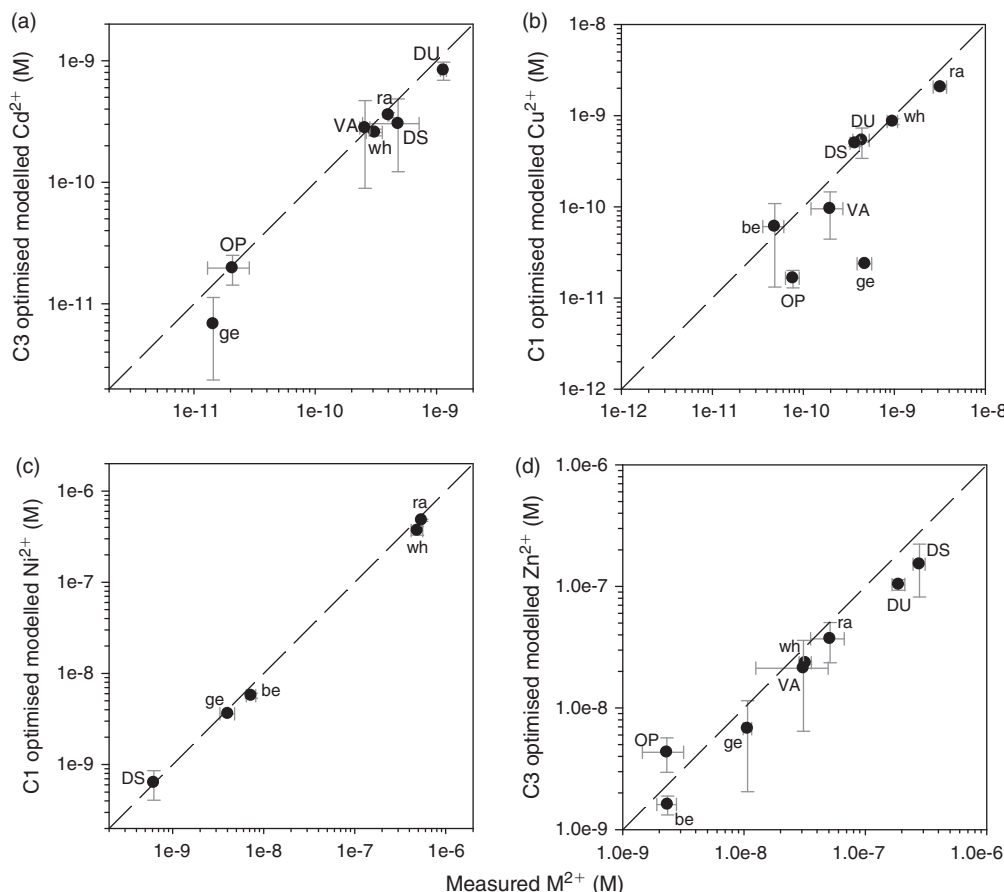
Fig. 4. Comparison of mean ( \pm s.d., n = 3 ) concentrations of the free metal ion [ M^{Z+} ] calculated with WHAM (with the percentage active fulvic acid (%aFA) estimated from Fig. 3) and those measured ( \pm s.d., n = 3 ) using the ion-exchange technique (IET) (Cd, Ni and Zn) or ion selective electrode (ISE) (Cu) methods: (a) cadmium; (b) copper; (c) nickel and (d) zinc. The dashed line represents the 1 : 1 line. The two-letter lake codes can be found in Table 1.
