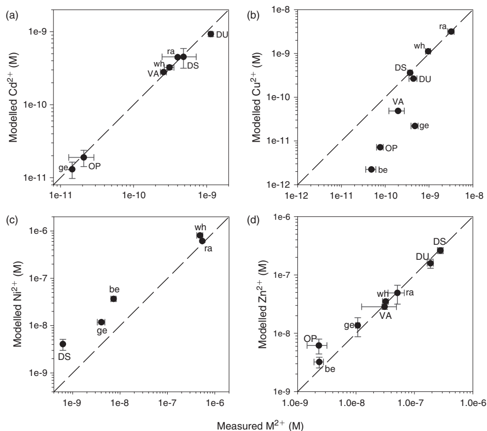
Fig. 1. Comparison of mean ( \pm s.d., n = 3 ) concentrations of the free metal ion [ M^{2+} ] calculated with WHAM (with the 65% active fulvic acid (aFA) assumption) and those measured using the ion exchange technique (IET) (Cd, Ni and Zn) and with an ion selective electrode (ISE) (Cu). The dashed line represents the 1 : 1 line. The two-letter lake codes can be found in Table 1.
