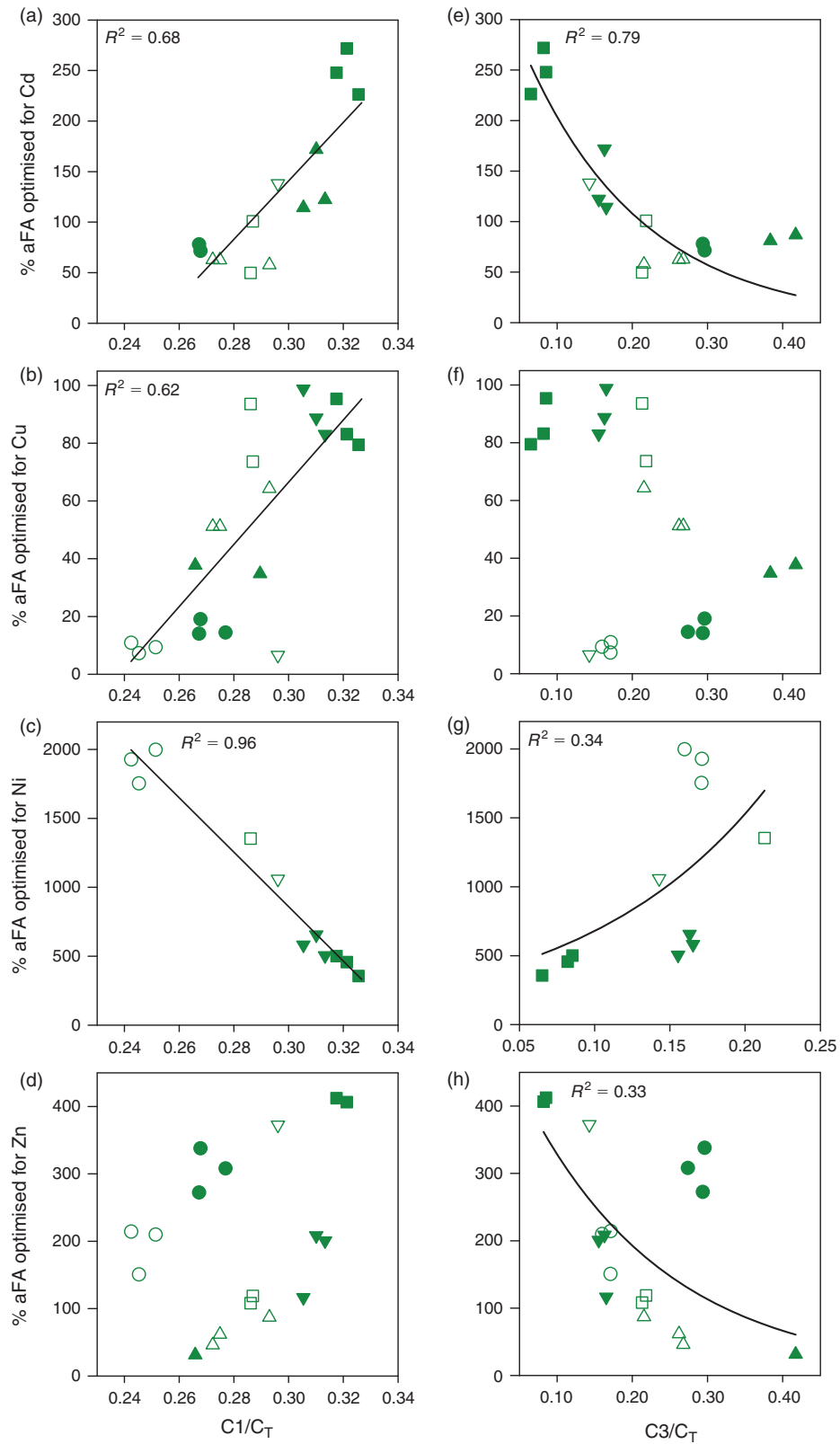
Fig. 3. Relationship between the WHAM calculated percentage fulvic acid active in complexation (%aFA opt ) for Cd, Cu, Ni and Zn and the relative contribution of parallel factor analysis (PARAFAC) fluorescence components 1 (panels a–d) and 3 (panels e–h) to the overall fluorescence spectrum of lake dissolved organic matter (DOM). Points of the same shape and fill represent replicate samples. Solid lines represent regression equations of statistical significance at the 0.05 \alpha -level.
