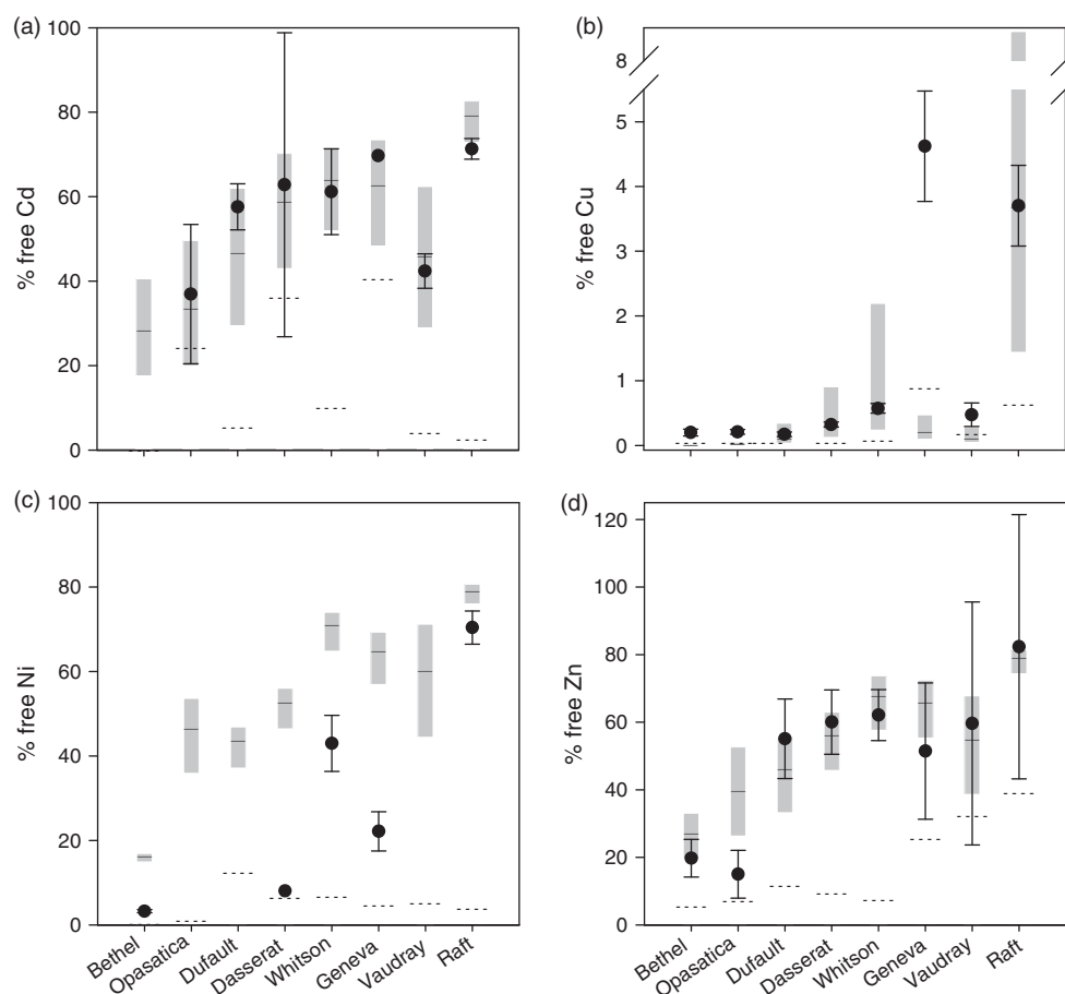
Fig. 2. Comparison between measured percentage of free Cd 2+ (a), Cu 2+ (b), Ni 2+ (c) and Zn 2+ (d) and WHAM predicted percentage of free M Z+ for eight lakes sampled from the regions of Rouyn-Noranda, QC and Sudbury, ON. Measured points below the method limit of quantification (LOQ) are not shown. WHAM predictions were calculated for a range of percentage active fulvic acid (%aFA) input values. Lakes on the x-axis are arranged from high pH on the left to low pH on the right. Solid circles are measured percentage of free M Z+ values with error bars representing standard deviation of triplicate measures. Grey vertical bars represent the range of WHAM predicted percentage of free M Z+ values using 33 to 130% active fulvic acid (aFA). Solid horizontal lines are WHAM predicted percentage of free M Z+ values using 65% aFA. Dashed horizontal lines represent the LOQ.
