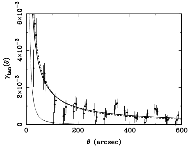
Figure 1 The mean shear, \gamma_{tan}(\theta) , around foreground galaxies in the g' , r' and i' bands, as measured by Fischer et al. (2000), is compared to various theoretical predictions. In each bin the data in the three bands (which are offset for clarity) are strongly correlated as the errors are dominated by the sample noise in the orientations of the background galaxies. The three models shown are: the best-fit power law (solid line); the MONDian prediction (dashed line); and the Newtonian result if there is no dark matter (dotted line).
