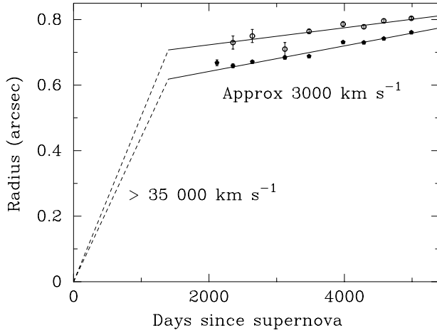
Figure 8 Inferred radius of the radio remnant SNR 1987A as a function of time. The filled points represent radii determined by fitting a thin spherical shell to the data, while open points correspond to a model involving a shell plus two point sources. The solid lines indicate the respective best-fit linear increases, while the dashed lines are extrapolations between the epoch of the supernova explosion and the time when radio emission re-appeared.
