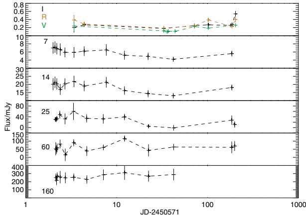
Figure 1 1997 variability of 3C 446 in log time.
