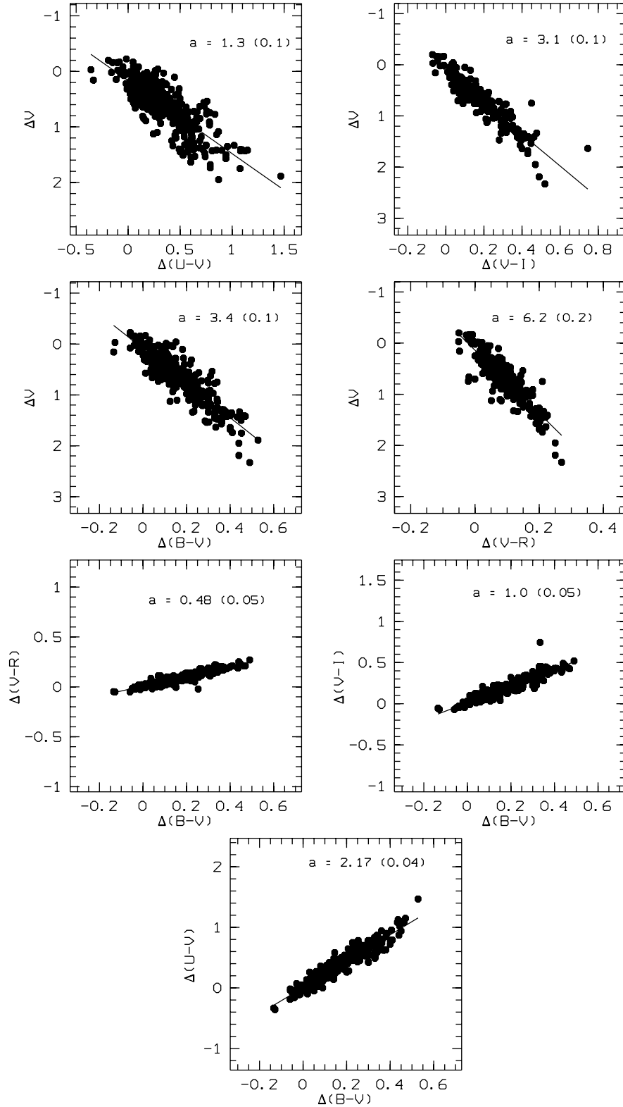
Figure 3 The adjusted zero point (see text) magnitude–colour and colour–colour diagrams for the recovery data for all RCB stars from this study. The slopes of the linear fit ( a ), with \sigma in brackets, are also given.
