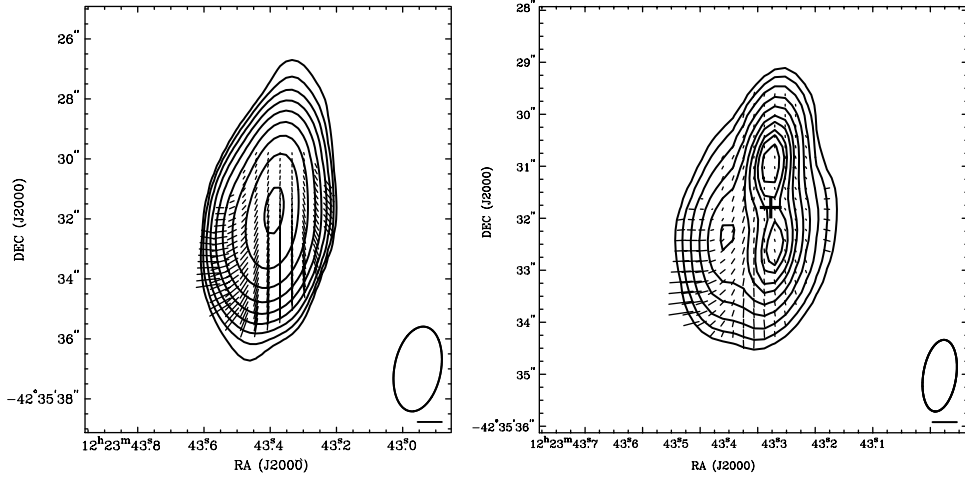
Figure 1 Left: 4.8 GHz total intensity contour map of B1221–423 with contours at 2, 4, 8, 16, 32, 64, 128, 256, 512 mJy beam −1 . Right: 8.6 GHz total intensity contour map of B1221–423 with contours at 3.75, 7.5, 15, 30, 50, 75, 100, 130, 150, 180 mJy beam −1 ; the cross marks the position of the optical nucleus. The restoring beam for each image is shown in the bottom right-hand corner of each panel. The vectors represent the observed E -vectors of the polarised emission with their length proportional to the fractional linear polarisation. The length of the vector corresponding to the maximum polarisation (9% at 4.8 GHz and 35% at 8.6 GHz) is given in the bottom right-hand corner.
