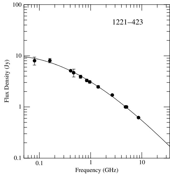
Figure 2 The radio spectrum of B1221–423. Data points are from the literature and from Table 1. A third order polynomial is fitted to the data.
