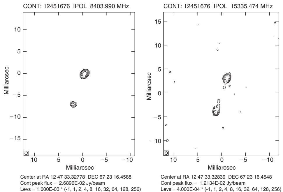
Figure 3 VLBI images of 1245+676 at 8.4 GHz (epoch 1991) and 15 GHz (epoch 1998).
