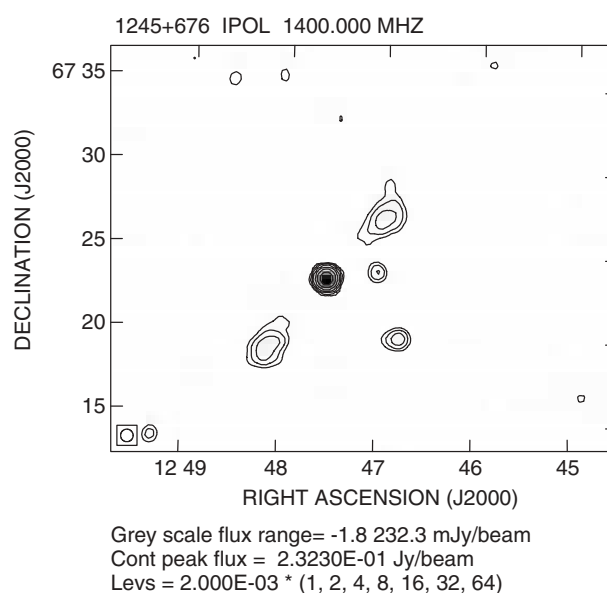
Figure 1 NVSS image of the whole structure of the radio galaxy 1245+676. The radio galaxy stretches SE–NW over 12''.4 — also two compact field sources are seen.
