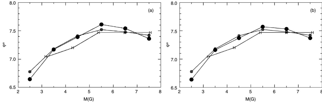
Figure 7 Logarithmic stellar luminosity function, implied by two model gradients: (a) GW and (b) BRK (●) overlaid with Gliese's (1969) (○) and Hipparcos' (JW 1997) (H) values.
