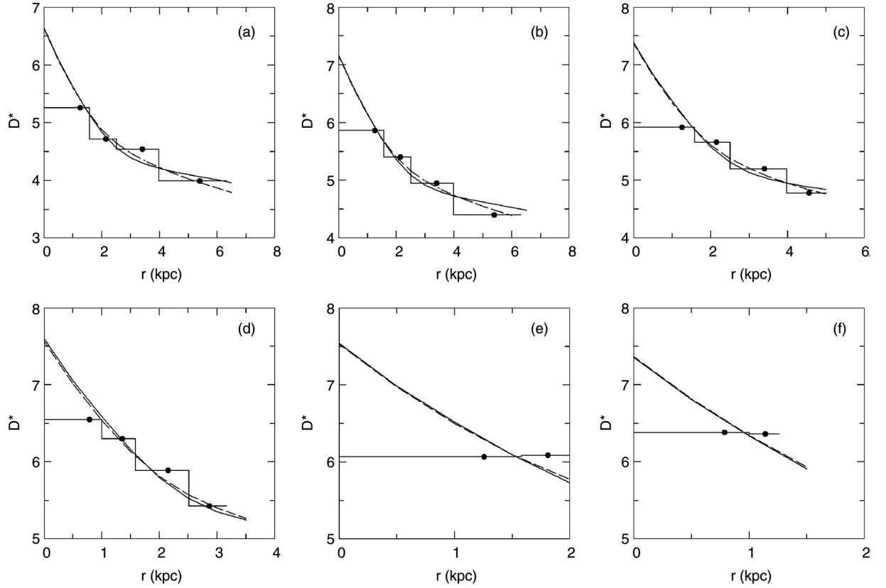
Figure 5 Logarithmic space-density histograms for all populations, within the limiting apparent magnitude of different M(G) intervals: (a) (2, 3] , (b) (3, 4] , (c) (4, 5] , (d) (5, 6] , (e) (6, 7] , and (f) (7, 8] . (●) centroid distances within the limits of completeness for comparison with BRK (dashed curve) and GW (thin curve) model gradients.
