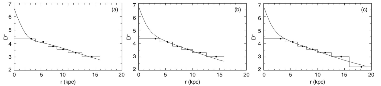
Figure 6 Logarithmic space-density histograms for giants for all populations ( M(G) \leq 2 mag), within the limiting apparent magnitude. (●) centroid distance within the limiting distance of completeness for comparison with two model gradients, i.e. (a) GW, (b) BRK, and (c) BRK for a larger distance interval ( r \leq 19.95 kpc).
