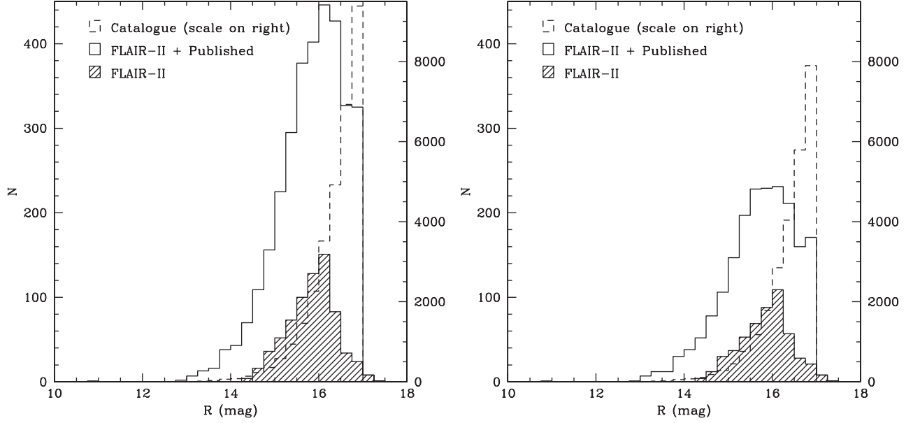
Figure 2 Magnitude distributions of observed and catalogued galaxies in the Shapley region. Left: full samples; Right: inter-cluster region only. Note that in each case the catalogue histogram is on a different scale, shown on the right.
