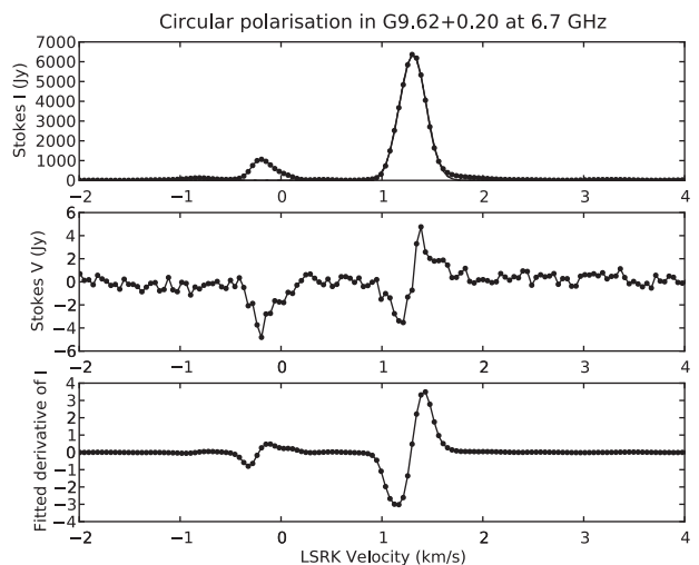
Figure 6 S-curve fitting for G9.62+0.20
