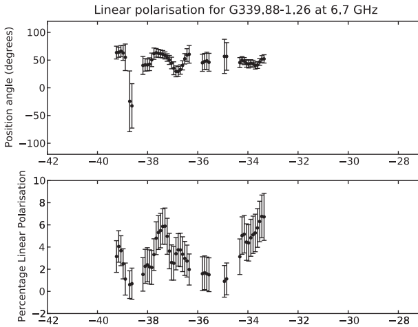
Figure 5 Percentage linear polarisation and position angle for G339.88–1.26, observations made during September 2010
