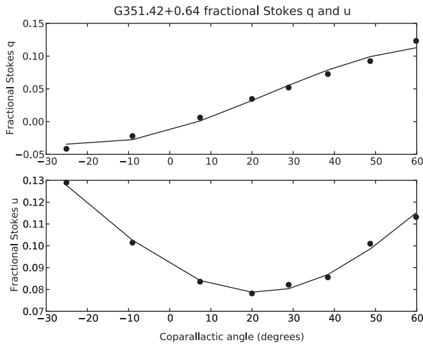
Figure 3 Fractional Stokes q and u against coparallactic angle with fit for G351.42+0.64
