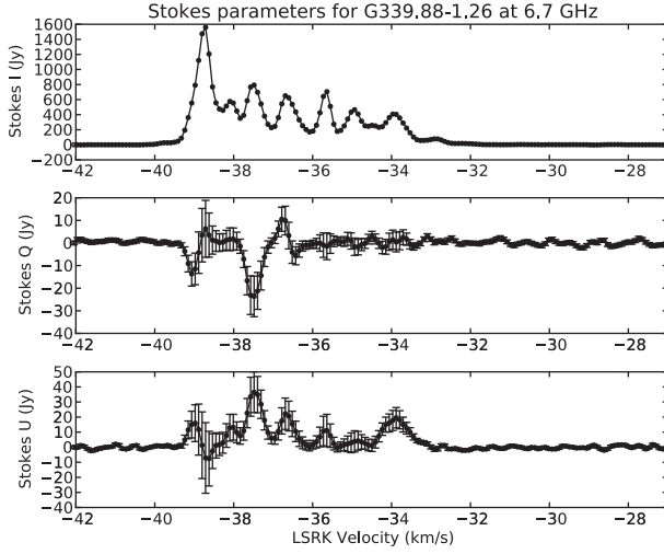
Figure 4 Stokes I, Q and U for G339.88–1.26, observations made during September 2010
