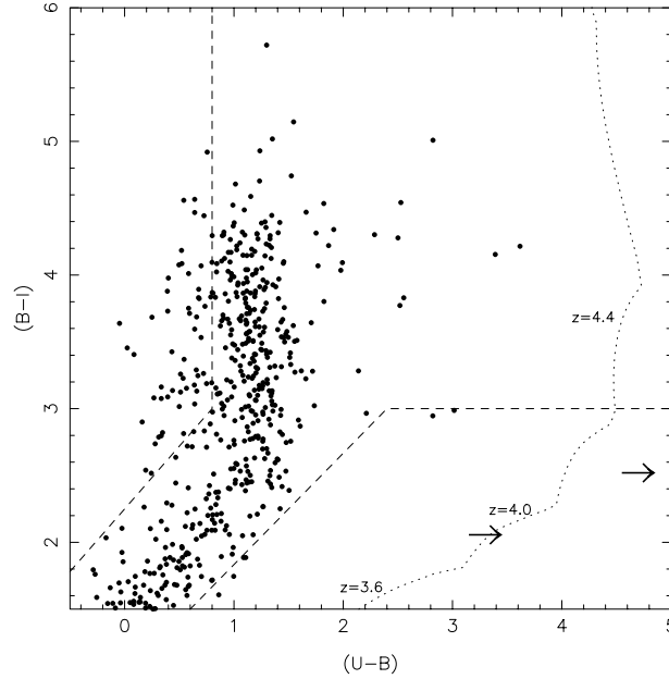
Figure 1 —The (U - B) – (B - I) colour–colour plot for the I < 21 objects with stellar morphologies from the combined fields of S98. The two QSOs are remarkable for their relatively blue (B - I) and very red (U - B) colours, and are marked as lower limits on this plot. The dotted line shows the expected colours of a QSO with a UV spectral slope of \nu^\alpha , with \alpha = 0.5 , as a function of redshift. This prediction includes the effects of blanketing by the Lyman- \alpha (Madau 1995). The structure in this locus arises from the approximations used in the blanketing estimate. We also show the rough boundaries of the region in the colour–colour plane within which stars fall (taken from the distribution in Landolt 1992).
