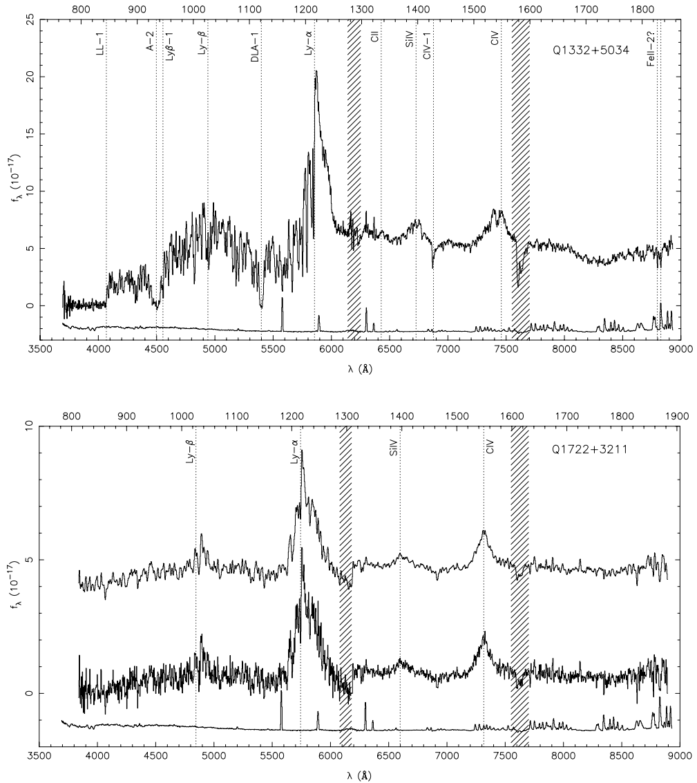
Figure 3 —The spectra of Q1332+5034 and Q1722+3211 obtained with ISIS on the WHT. Each panel shows the fluxed spectrum of the source, as well as an arbitrarily scaled spectrum of the night sky. In addition, in Q1722+3211, we also show at the top the spectrum smoothed to the instrumental resolution. The identifications of the main features are shown in both spectra (Table 2). In Q1332+5034 the features marked with -1/-2 are associated with the foreground absorption systems. The lower scale on each plot gives the observed wavelengths, while the upper scale indicates the wavelengths in the rest frame of the QSO. The hatched regions mark areas affected by atmospheric absorption or the dichroic of the spectrograph.
