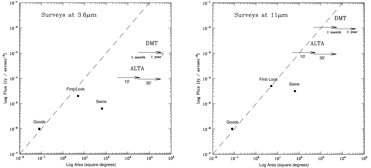
Figure 1 Parameter space for galaxy number counts studies that could be explored by Antarctic telescopes working at 3.6 \mu\text{m} and 11 \mu\text{m} . Plotted, as a function of the achievable sensitivity (in \text{Jy}/\text{arcsec}^{-2} ), is the sky coverage in square degrees that could be surveyed by the 2 m DMT and the 6.5 m ALTA. For each telescope, the arrow shows the area covered if the field of view was 10' (left) and 30' (right). The length of the arrow shows the range in areal coverage if the observing time varies from 1 month to 1 year (with a 33% assumed observing efficiency). The dashed line shows the relation for equivalent surveys (i.e. total number of sources detected) if the number of sources were inversely proportional to their flux. Also shown are the anticipated coverage/flux limit of three surveys planned for the SIRTf space telescope; 'Goods', 'First Look' and 'Swire'. Note that the DMT survey at 3.6 \mu\text{m} with a 30' FOV is truncated when complete sky coverage is reached (which requires just 1.5 months).
