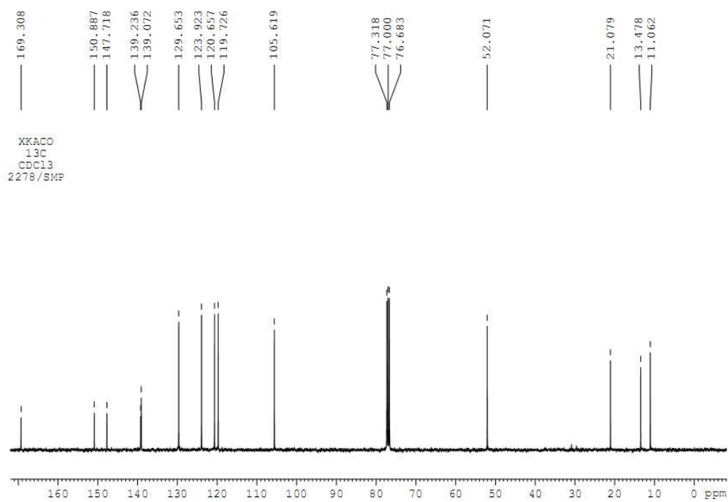
^{13}\text{C} NMR spectrum of ligand 1b
