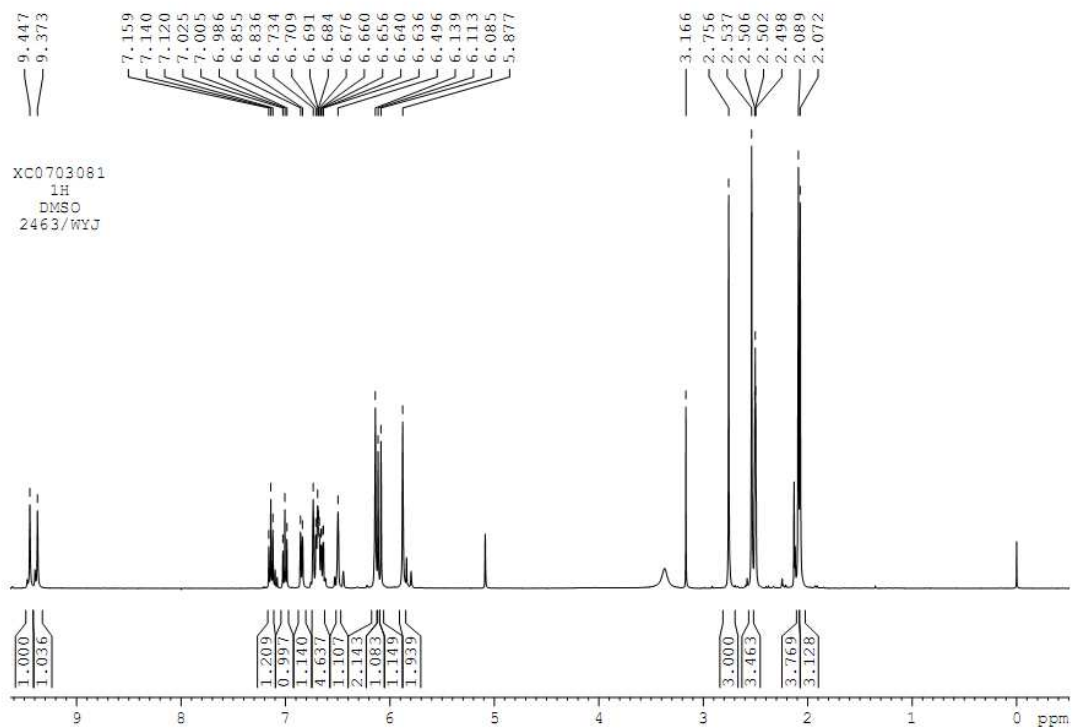
1 H NMR spectrum of complex 2a
