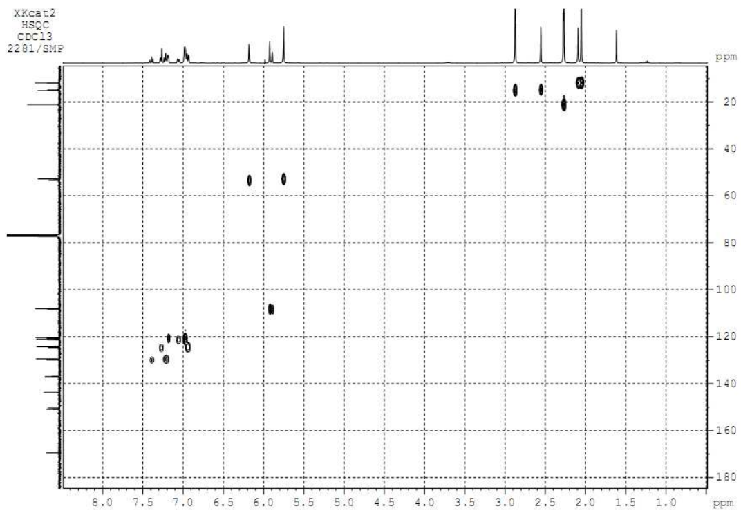
C-H COSY spectrum of complex 2b after the sample solution was placed at rt for 3-4 days
