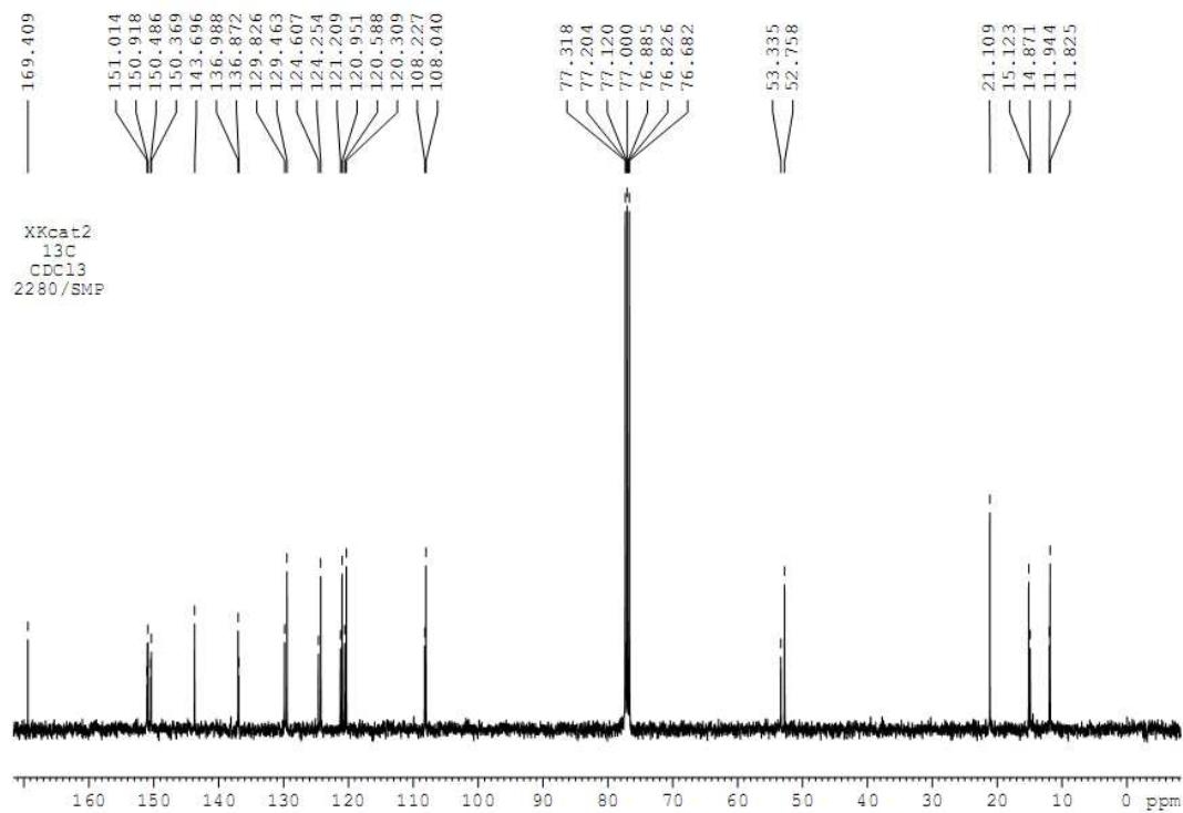
13 C NMR spectrum of complex 2b after the sample solution was placed at rt for 3-4 days
