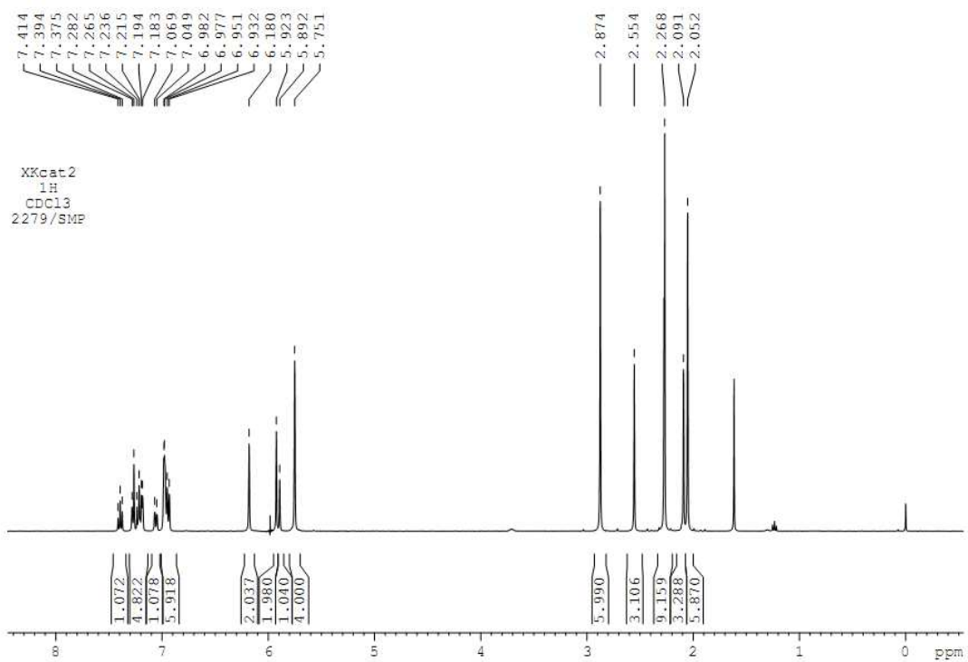
1 H NMR spectrum of complex 2b after the sample solution was placed at rt for 3-4 days
