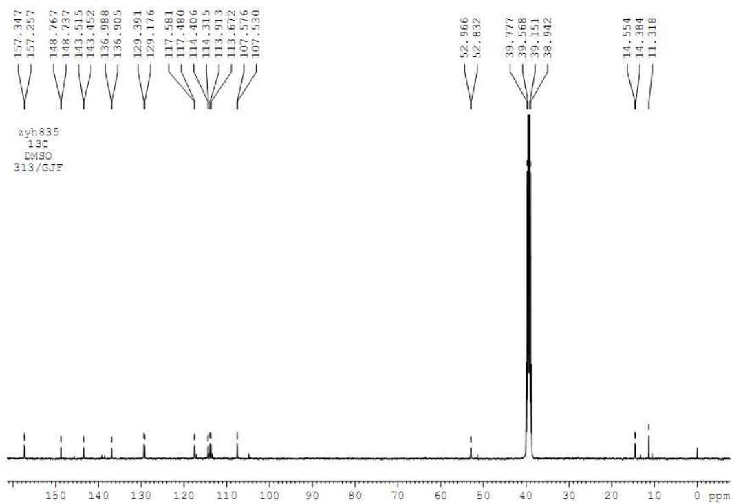
13 C NMR spectrum of complex 2a
