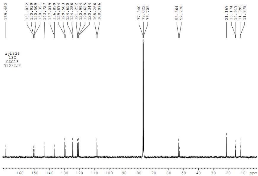
13 C NMR spectrum of complex 2b
