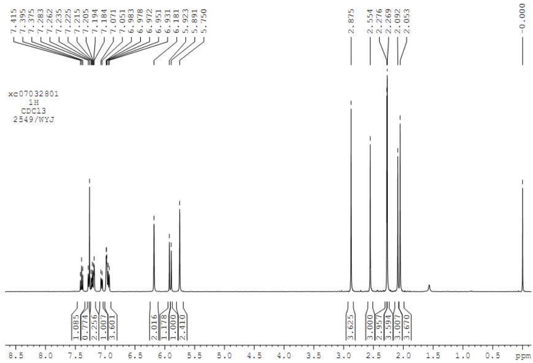
1 H NMR spectrum of complex 2b
