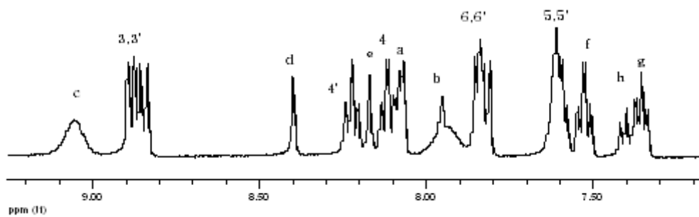
Fig. S1. The comparisons of downfield ^1\text{H} NMR spectra of Htip (a) and [\text{Ru}(\text{bpy})_2(\text{Htip})](\text{PF}_6)_2 . A proton-numbering scheme is shown on the top.
