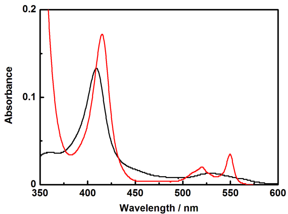
Fig. S1. UV-vis spectra of oxidised Cyt. c (black line) and reduced Cyt. c (red line) in phosphate buffer.
