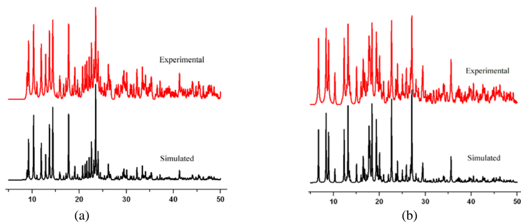
Fig.S1 XRPD for complexes (a) Complex 1; (b) Complex 2.
