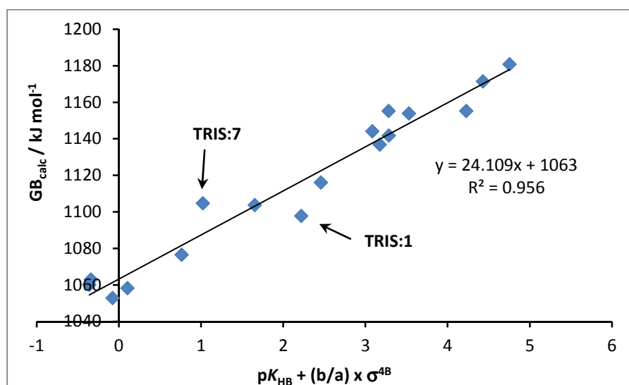
Figure S5. Correlation of the GBs calculated for TRIS series of bases against two independent variables pK_{HB} and \sigma^{4B}
