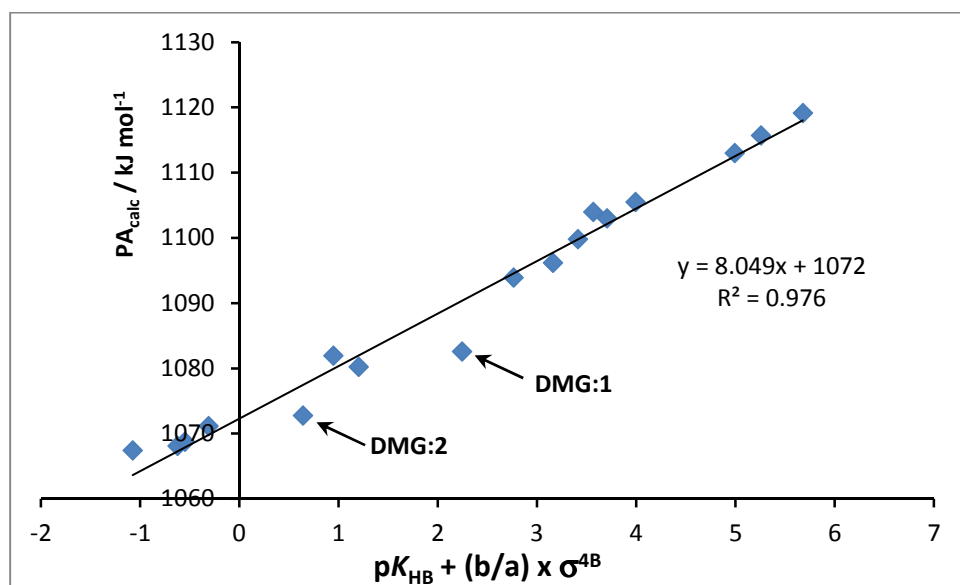
Figure S6. Correlation of the PA calculated for DMG series of bases against two independent variables pK_{HB} and \sigma^{4B}
