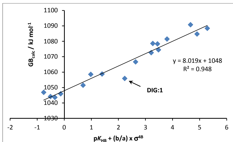
Figure S4. Correlation of the GB calculated for DIG series of bases against two independent variables pK_{HB} and \sigma^{4B}
