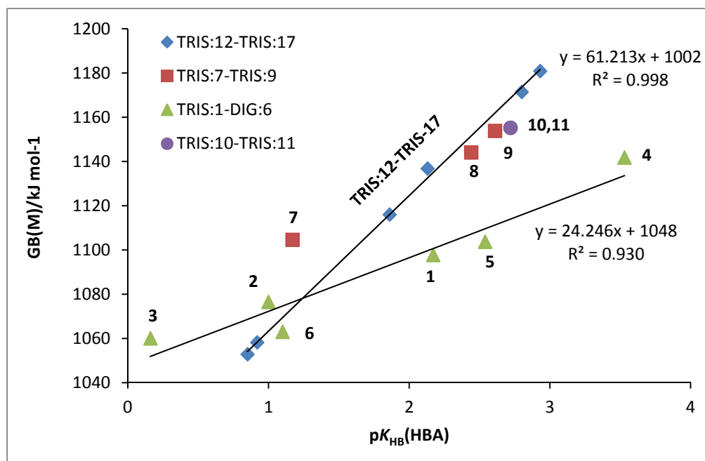
Figure S3. Correlation of the calculated gas-phase basicity (GB) against pK_{HB} (HBA) in TRIS series of bases. M = \text{TRIS}:X where X = 1-17 .
