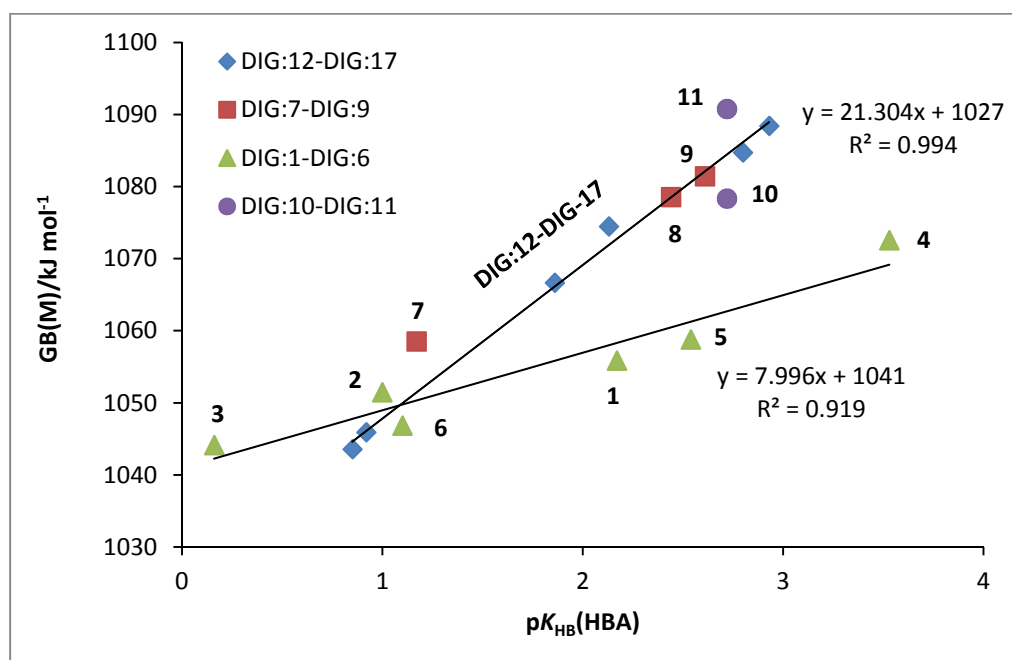
Figure S2. Correlation of the calculated gas-phase basicity (GB) against pK_{HB} (HBA) in DIG series of bases. M = \text{DIG}:X where X = 1-17 .
