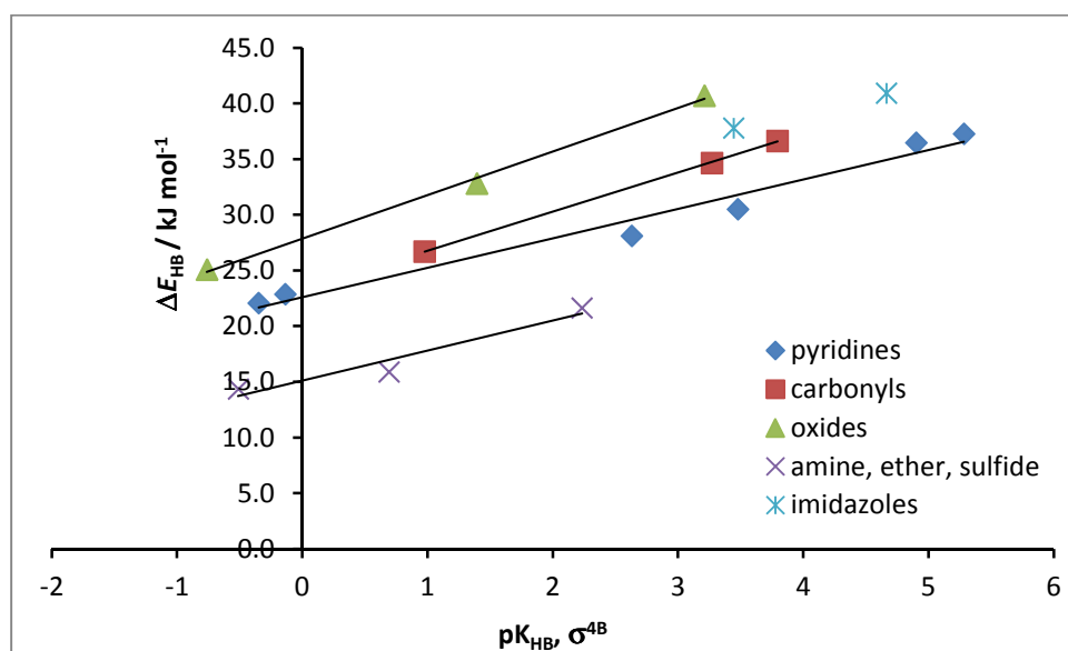
Figure S8. Correlation of the \Delta E_{\text{HB}} calculated for DIG series of bases against two independent variables \text{p}K_{\text{HB}} and \sigma^{4\text{B}} as used for the correlation of GBs.
