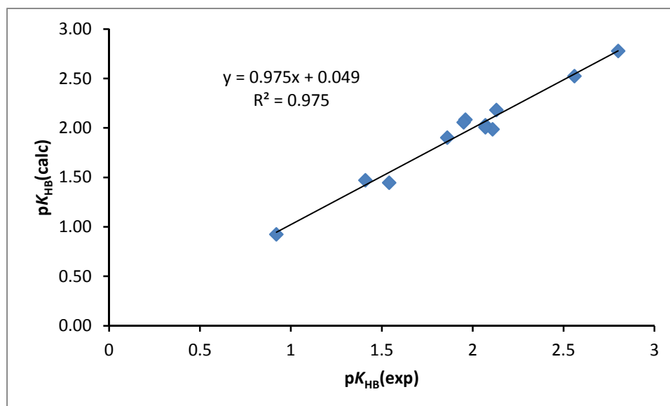
Figure S1. Correlation of the pK_{HB}(\text{calc}) calculated according eq. (S1) against experimental pK_{HB} [3] used for the evaluation of pK_{HB} (4-nitropyridine).
