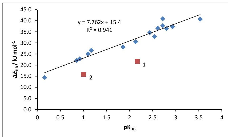
Figure S7. Correlation of the \Delta E_{\text{HB}} calculated for DIG series of bases against two independent variables \text{p}K_{\text{HB}} .
