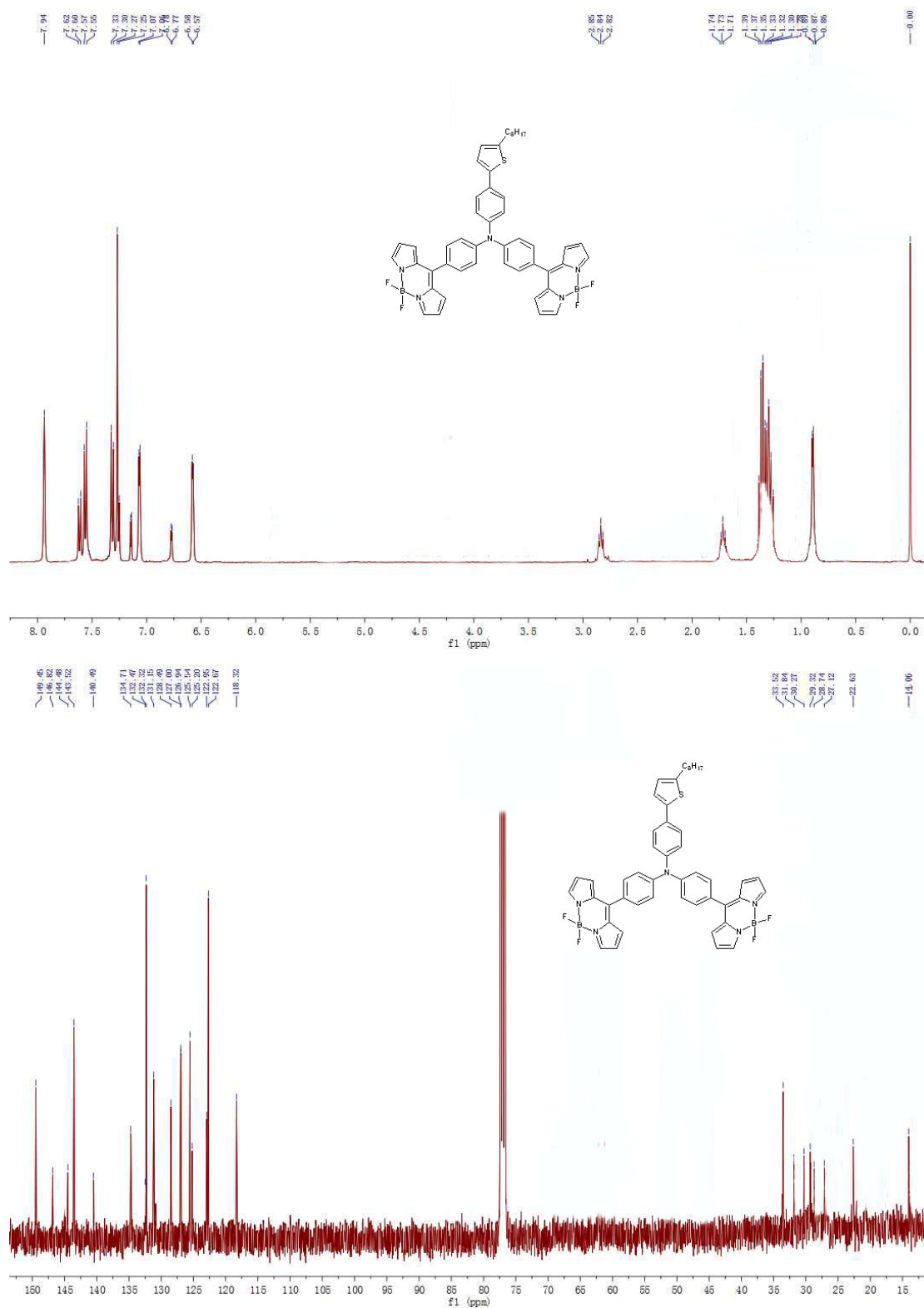
1 H NMR and 13 C NMR spectra of compound BDP8 .
