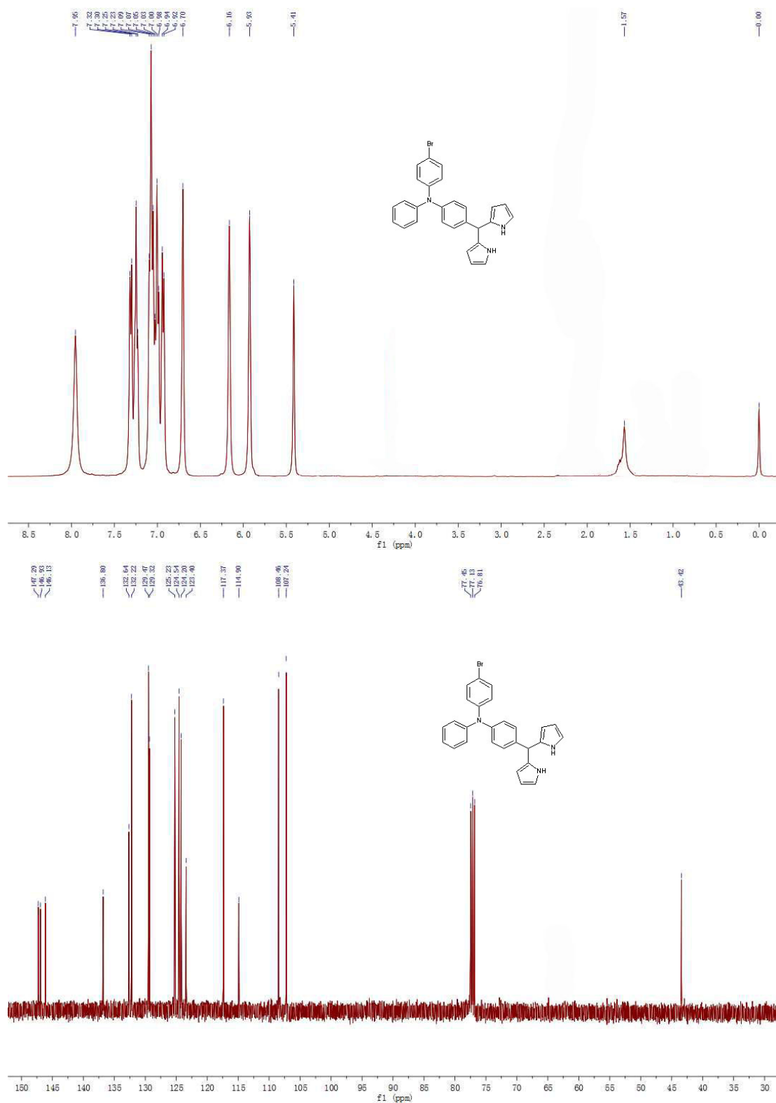
^1\text{H} NMR and ^{13}\text{C} NMR spectra of compound 6 .
