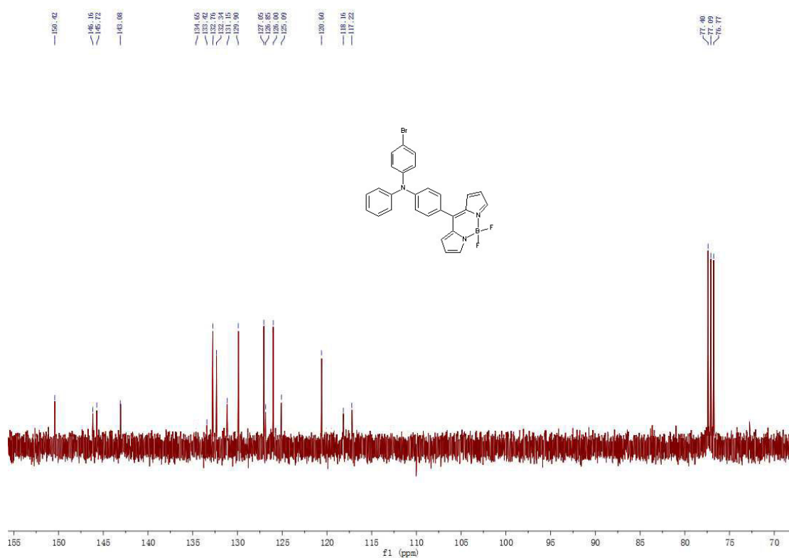
1 H NMR and 13 C NMR spectra of compound BDP5 .
