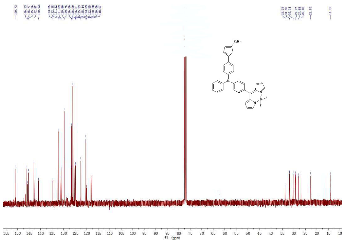
1 H NMR and 13 C NMR spectra of compound BDP7.
