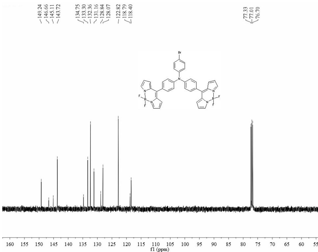
^1\text{H} NMR and ^{13}\text{C} NMR spectra of compound BDP6 .
