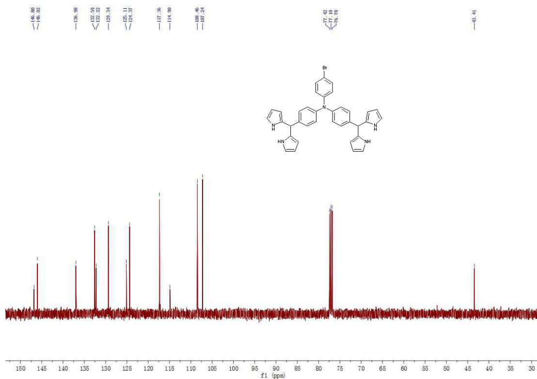
^1\text{H} NMR and ^{13}\text{C} NMR spectra of compound 8 .
