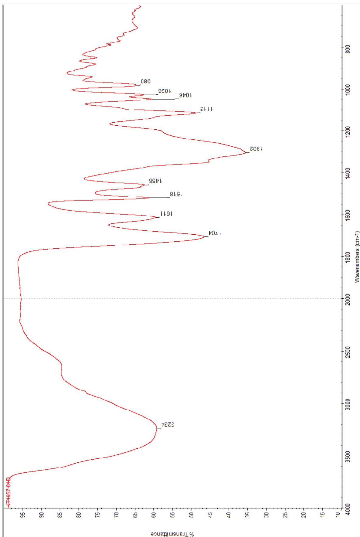
Infrared spectrum of 3
