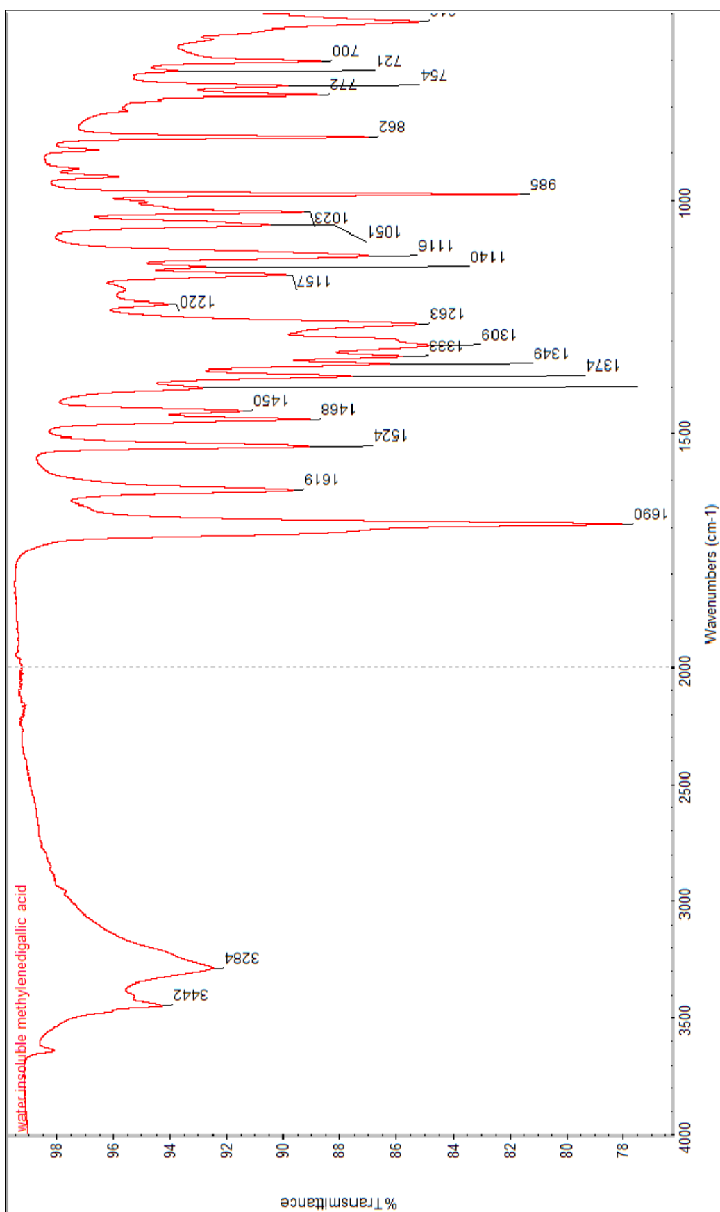
Infrared spectrum of 2
