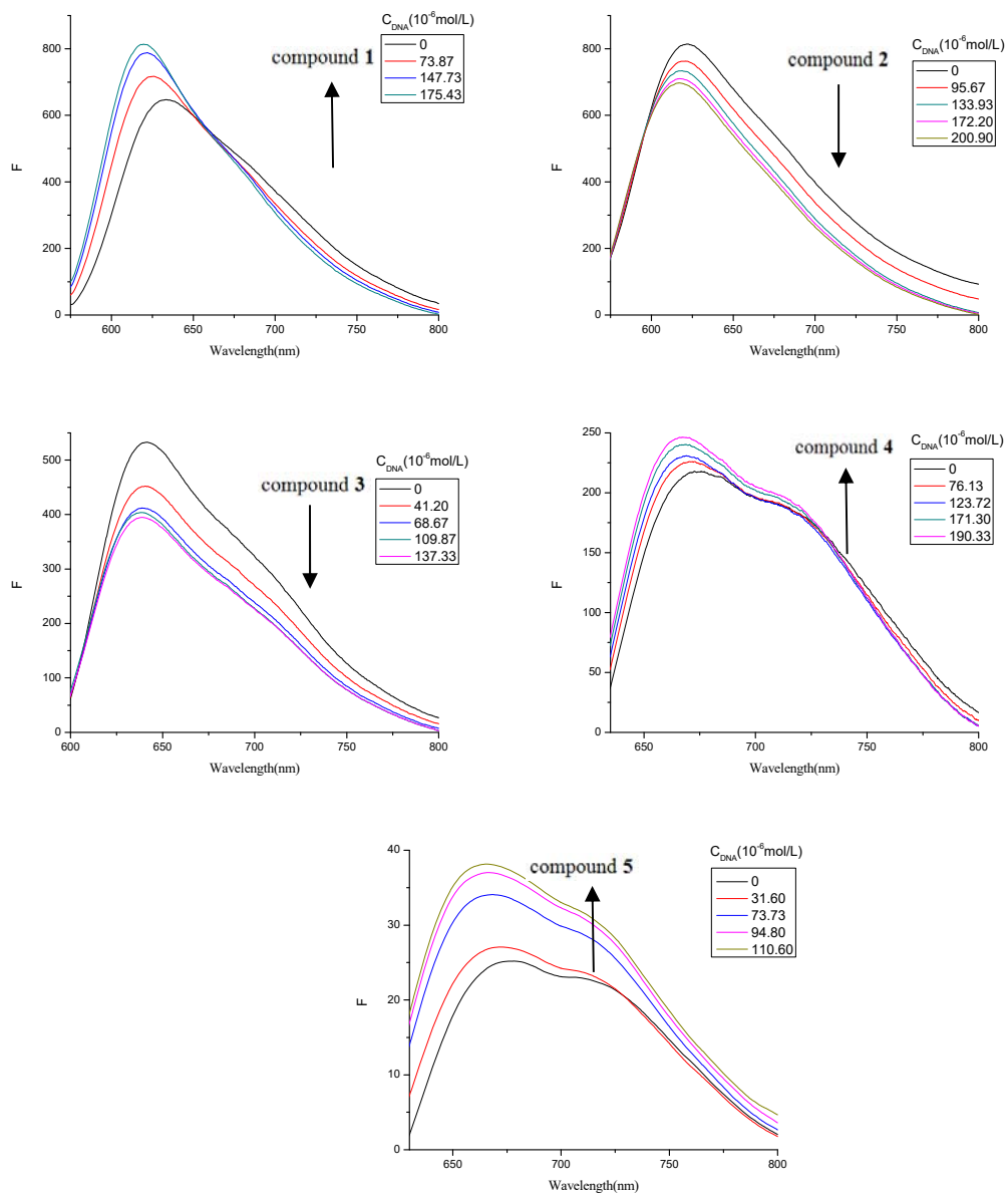
Figure S1. Fluorescence spectra of compounds 1-5 with the titration of CT DNA
