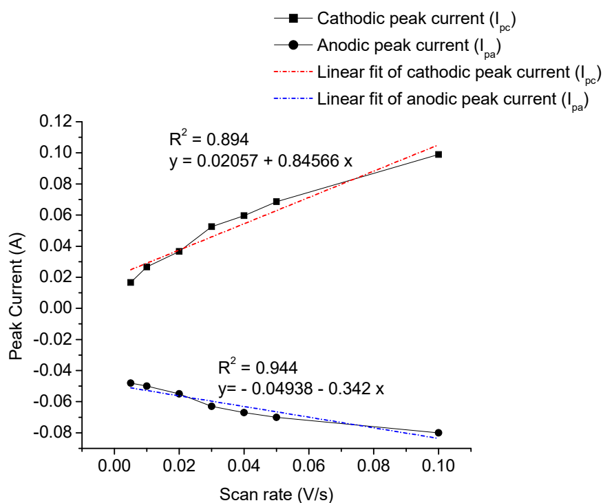
Fig. S1. Plot of cathodic and anodic peak currents as a function of scan rate.
