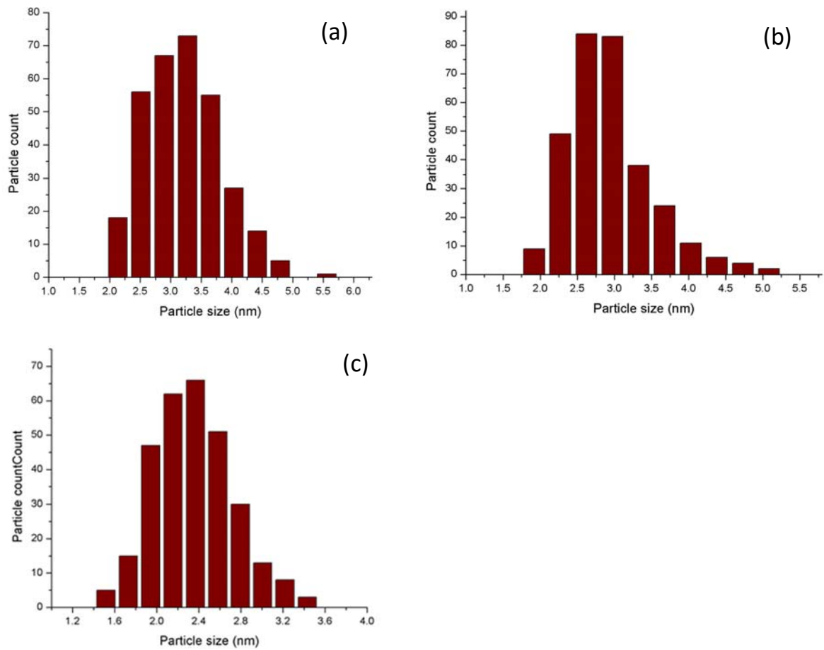
Figure S1 Histogram of particle size distribution for a) ZnO/MEA, b) ZnO/DEA and c) ZnO/TEA
