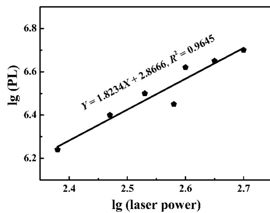
Fig. S2 Relation between the emission intensity and excitation laser power of the upconversion spectra of orpiment QDs.
