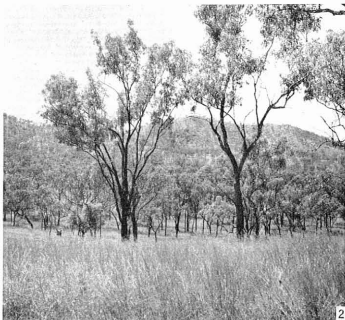
Fig. 2.—Narrow-leaved ironbark-red-barked bloodwood Open Forest is characteristic of most of the hilly country.
