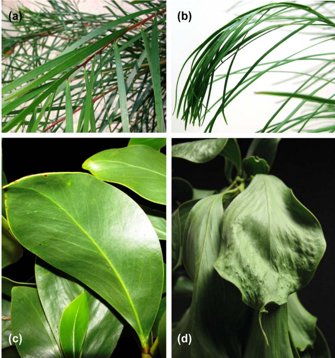
Fig. S1. Loss of turgor in (a, b) Acacia floribunda and (c, d) A. pycnantha phyllodes. (a, c) Phyllodes from well-watered plants, (b, d) phyllodes from droughted plants on day of greatest water stress.
