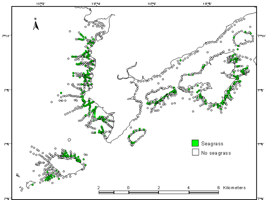
Figure S1. Seagrass survey sites near Banggi Island.
