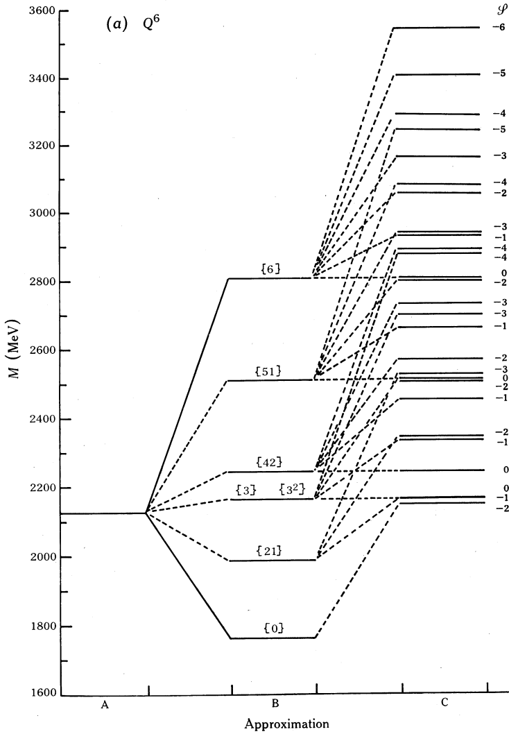
Figs 1a and 1b. Calculated masses for the S -wave colour singlet states of the quark configurations (a) Q^6 and (b) Q^9 . The strangeness number \mathcal{S} associated with each state is indicated. The approximations represented are (see text):
