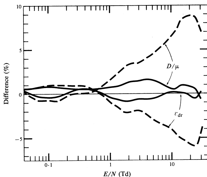
Fig. 18. Differences between the measured values of v_{dr} and D_T/\mu in H 2 and those calculated using the theoretical cross sections (dashed curves). The corresponding differences when the swarm-derived cross sections are used (full curves) are shown for comparison.
