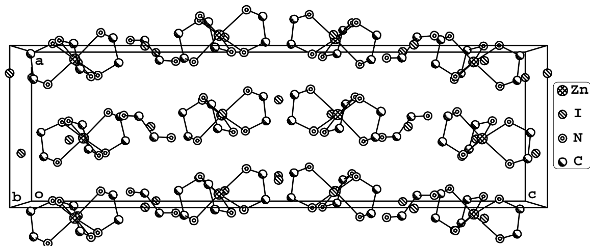
Fig.S1. Packing diagram of 1.
