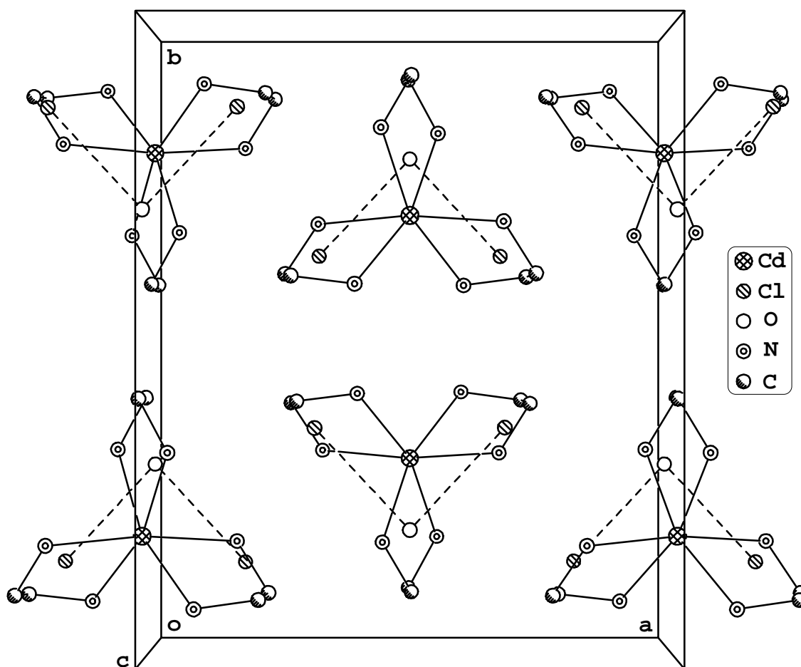
Fig.S1. Packing diagram of 1.
