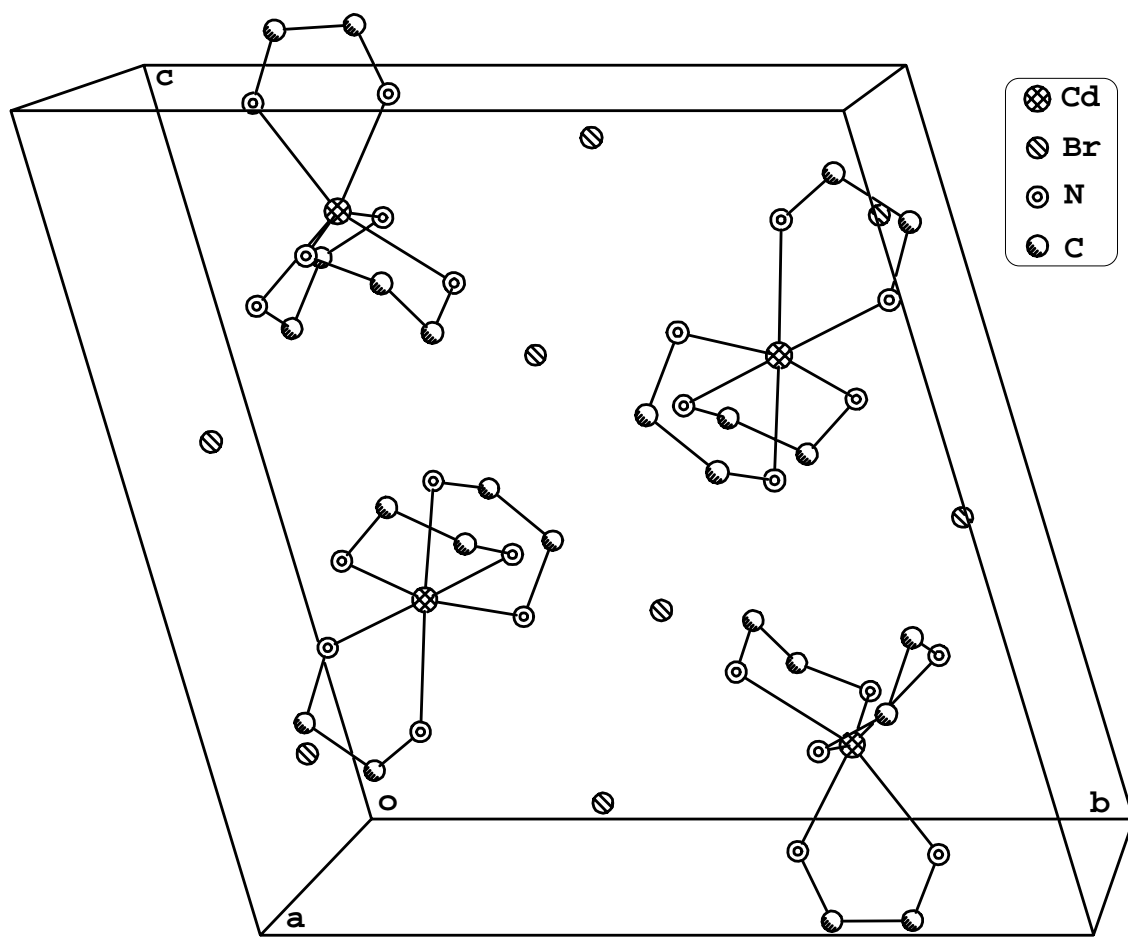
Fig.S3.Packing diagram of 3.
