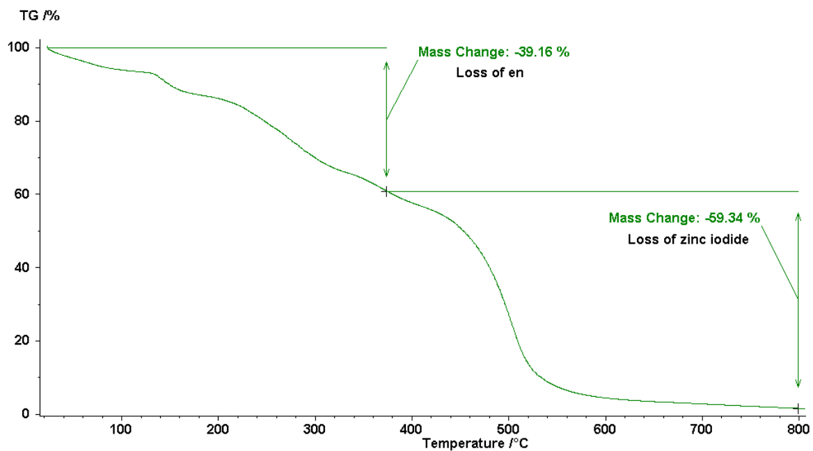
Fig.S4.TGA curve showing weight loss of 1.
