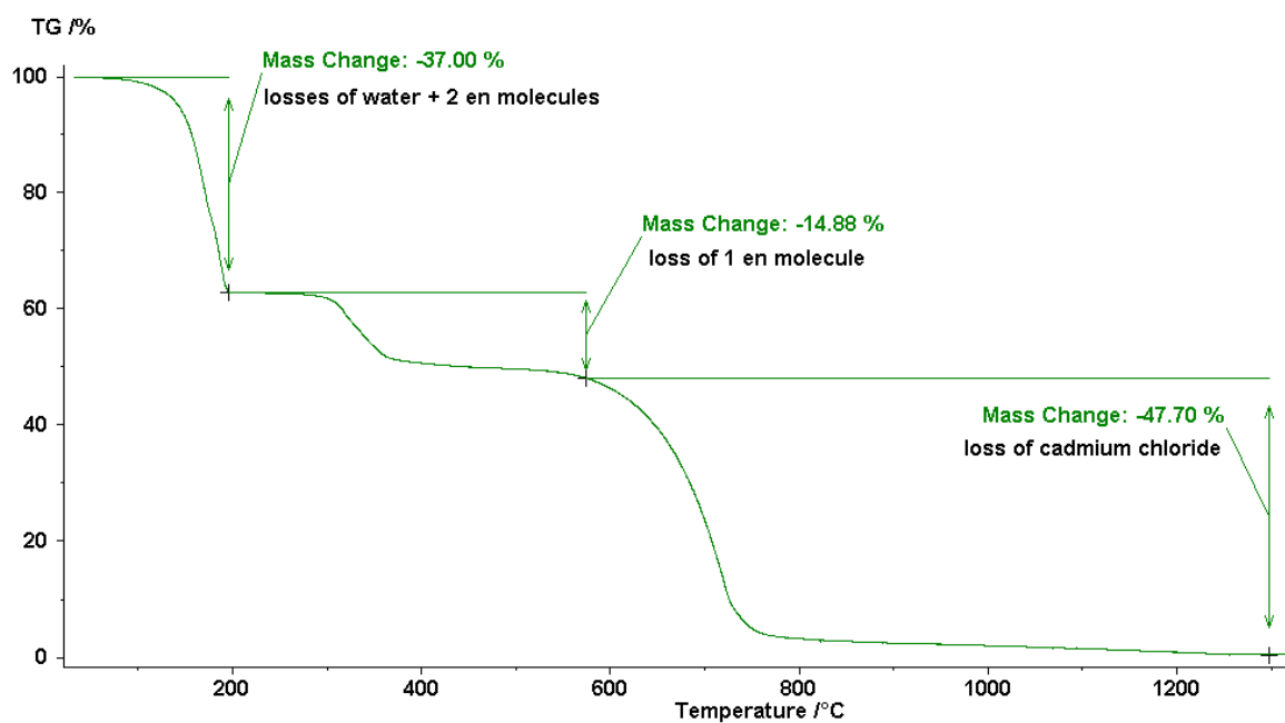
Fig.S5.TGA curve showing weight loss of 2.
