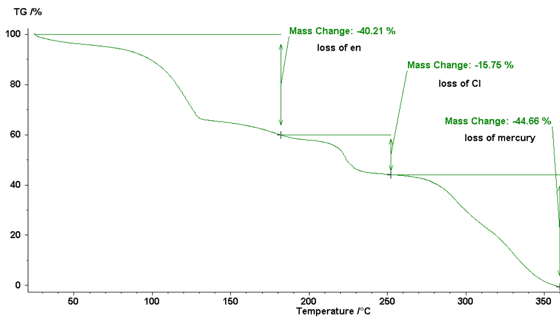
Fig.S7.TGA curve showing weight loss of 4.
