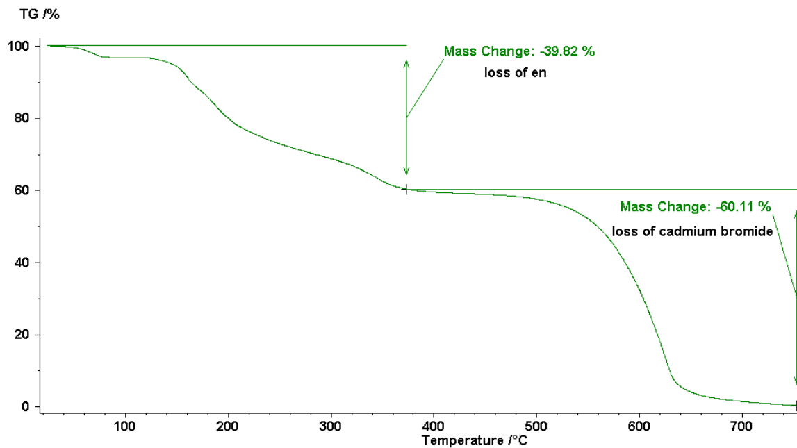
Fig.S6.TGA curve showing weight loss of 3.
