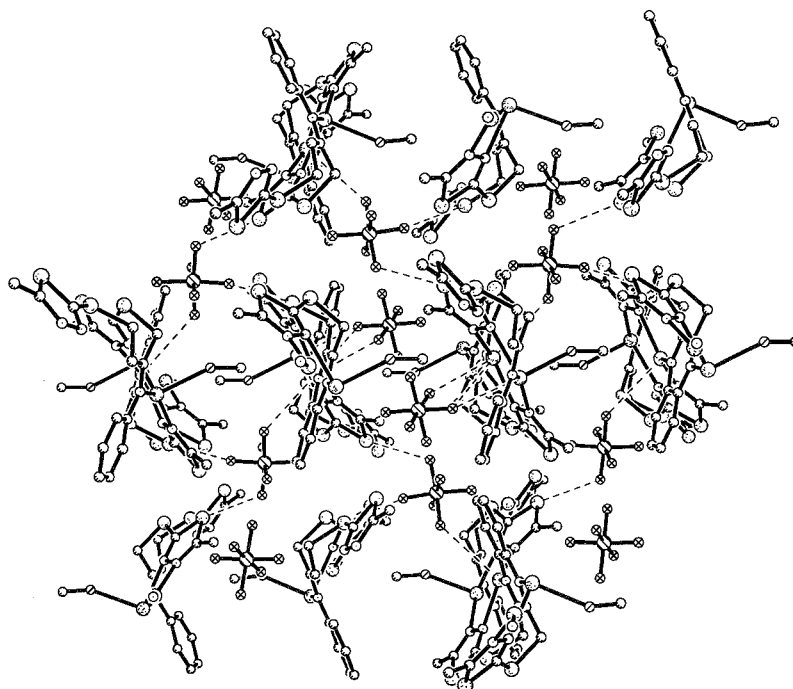
Fig. S2. The 3D supramolecular structure formed through the weak F...S interactions in 2 .
