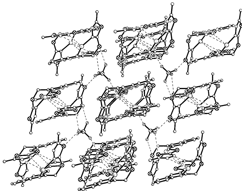
Fig. S1. The 3-D supramolecular structure formed through the weak O...S interactions in 1 .
