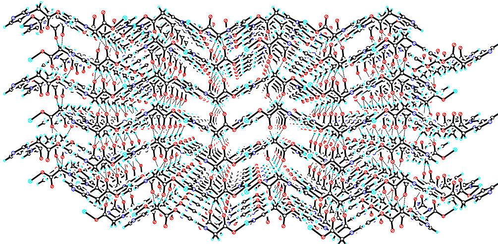
Fig. A3. Perspective of molecular packing in 3 along a axis. The dashed lines stand for hydrogen bond.
