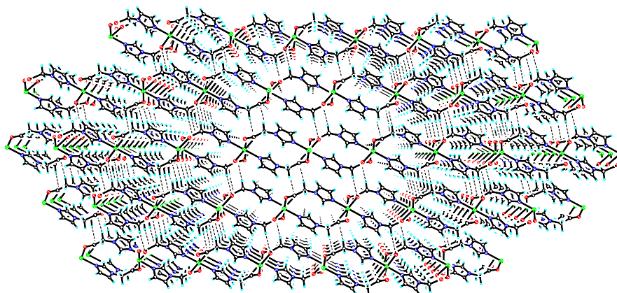
Fig. A2. Perspective of molecular packing in 2 (bottom) along [010] direction. The dashed lines stand for hydrogen bond.
