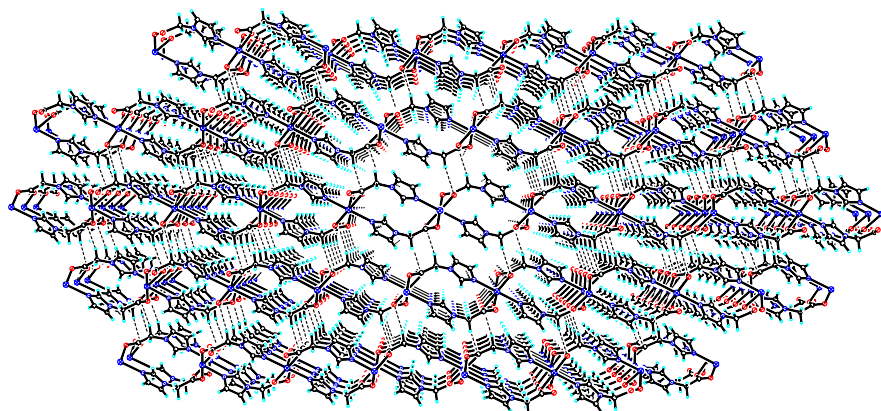
Fig. A1. Perspective of molecular packing in 1 along [010] direction. The dashed lines stand for hydrogen bond.
