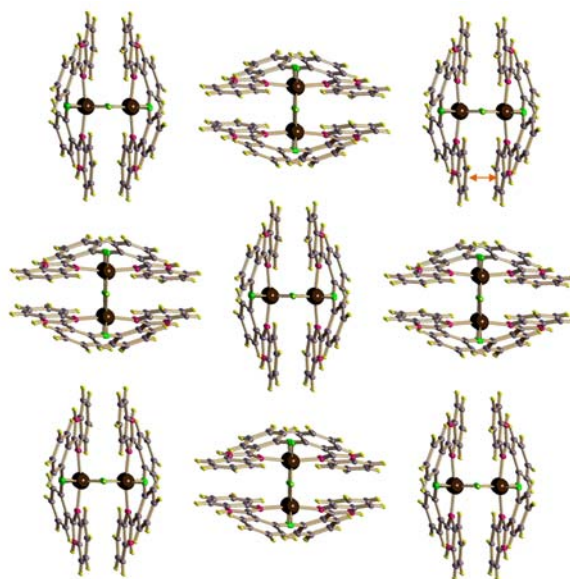
Figure A3. The molecular packing pattern in 1 and 2 . The inter-planar distance for the intramolecular \pi - \pi interaction is ca. 3.31 and 3.57 Å, respectively. For clarity, the lattice ethanol and water molecules are omitted.
