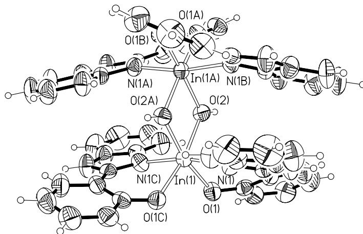
Figure A1. Perspective view of the molecular structure of 2 . Thermal ellipsoids are plotted at the 50 % probability level. Symmetry codes: A 1-x, 1-y, z; B 1-y, 1-x, -z; C y, x, -z.
