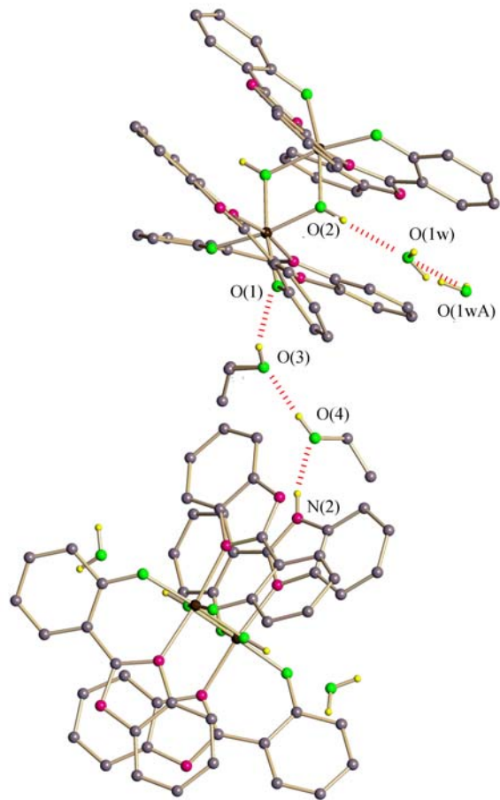
Figure A2. Perspective view of hydrogen bond interactions in 1 and 2 .
