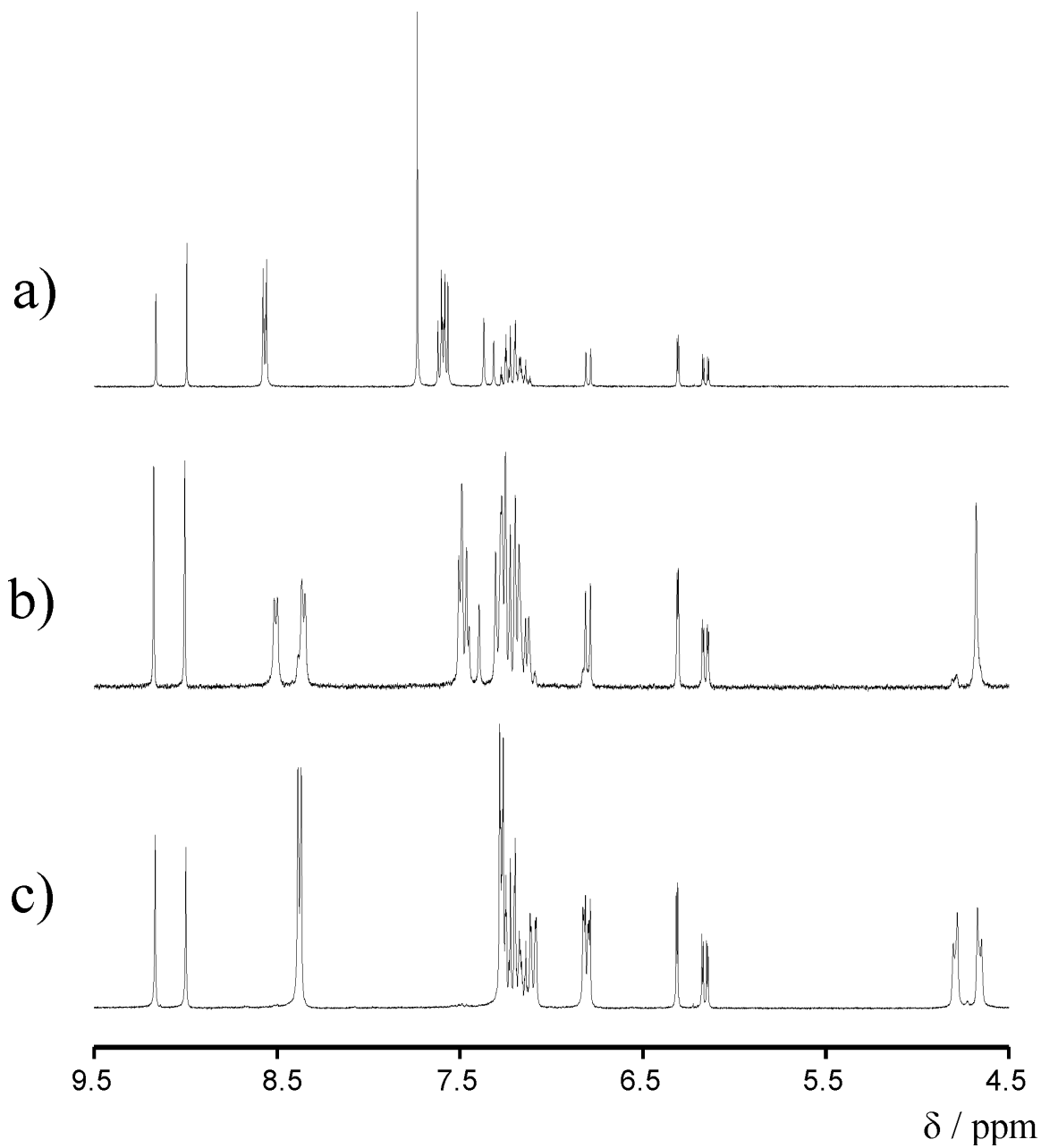
Figure F1. ^1\text{H} NMR spectra of cocrystals of 2(2)·2(3): a) before irradiation; b) after 36 hours irradiation with 420 nm wavelength radiation and c) after 48 hours irradiation with light from a 500 W high-pressure broadband mercury lamp.
