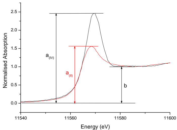
Supplementary Figure S2. Example XANES spectra of Pt(II) and Pt(IV) complexes, showing the difference in peak heights for the two oxidation states, and the parameters a and b used in determining the ratio a/b . Note the greater degree of absorption in the white line height of Pt(IV) complexes.
