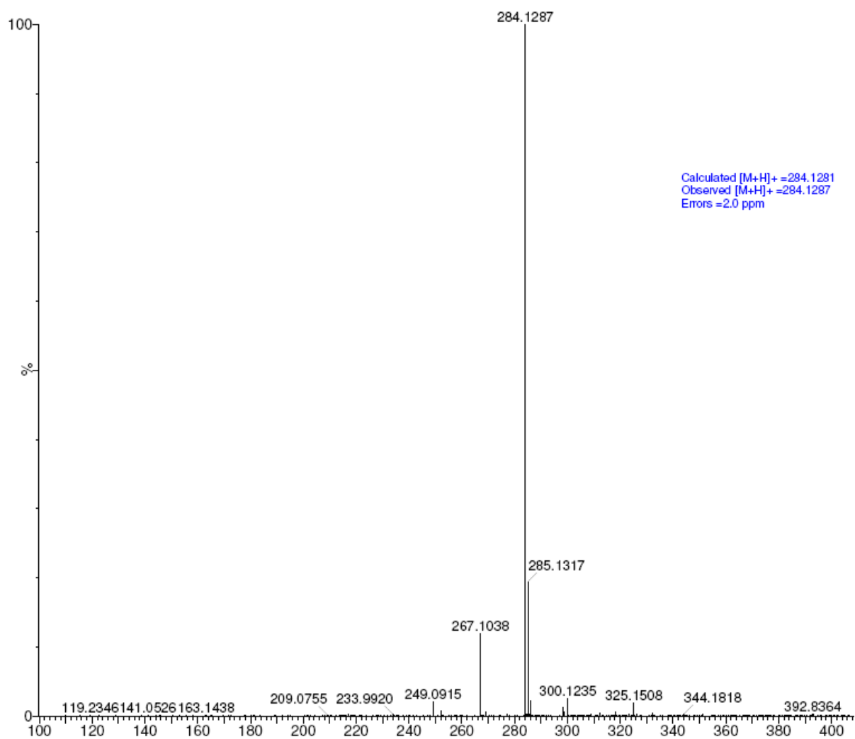
Figure 9. High Resolution MS of N -Nororipavine
