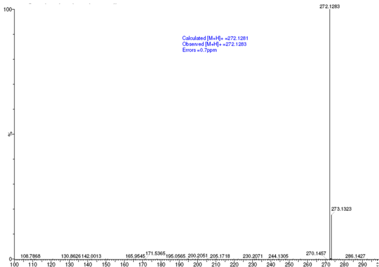
Figure 3. High Resolution MS of N -Normorphine
