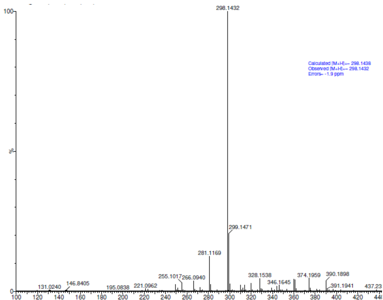
Figure 12. High Resolution MS of N -Northebaine
