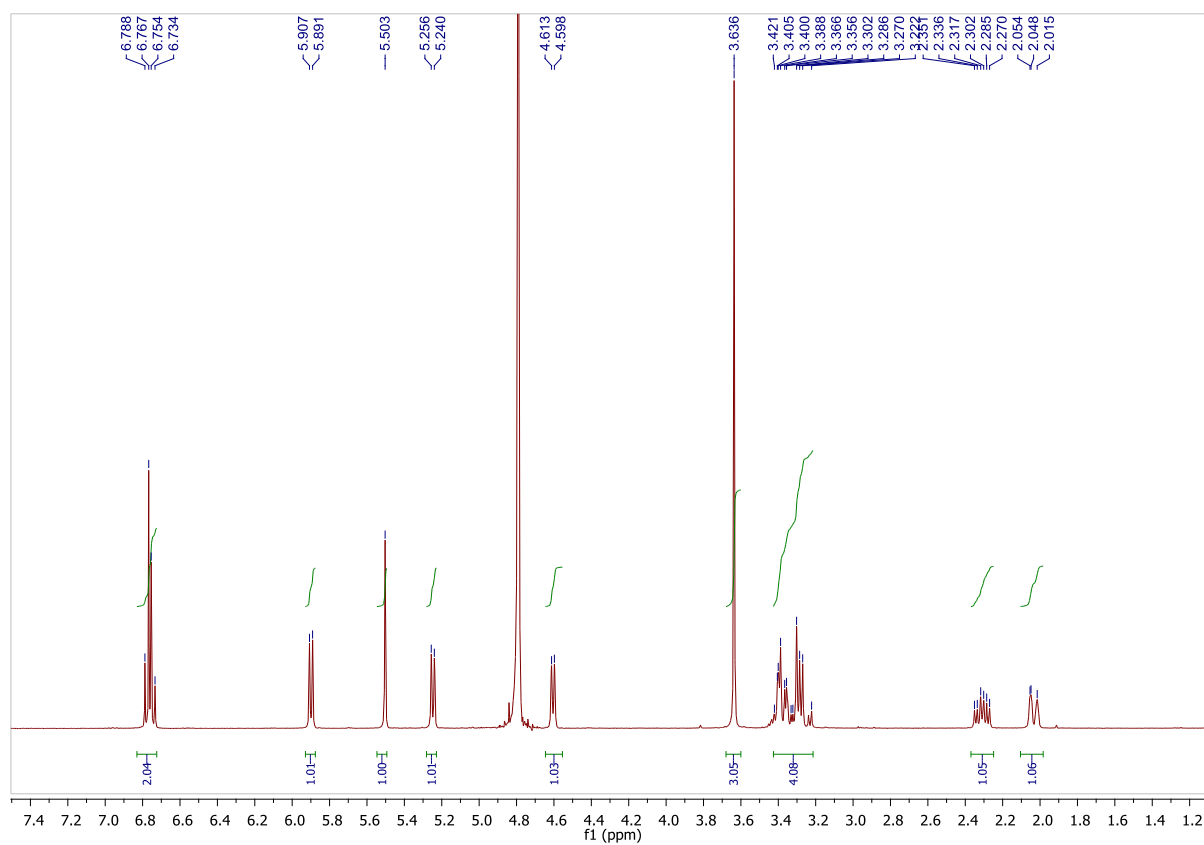
Figure 7. ^1\text{H} NMR spectrum of N -Nororipavine Hydrochloride in \text{D}_2\text{O}
