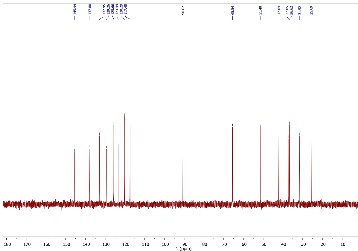
Figure 2. ^{13}\text{C} NMR spectrum of N -Normorphine Hydrochloride in \text{D}_2\text{O} + \text{TFA}
