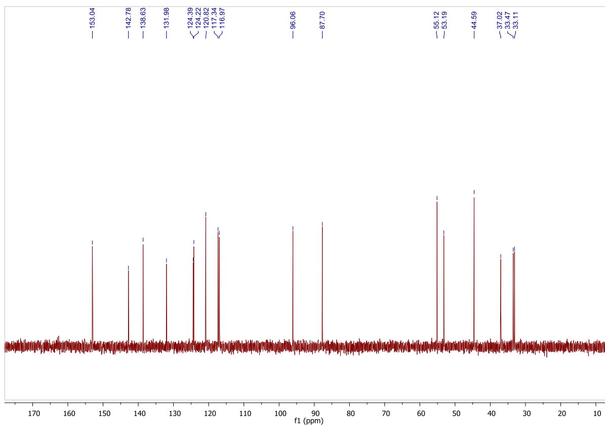
Figure 8. ^{13}\text{C} NMR spectrum of N -Nororipavine Hydrochloride in \text{D}_2\text{O} + \text{TFA}
