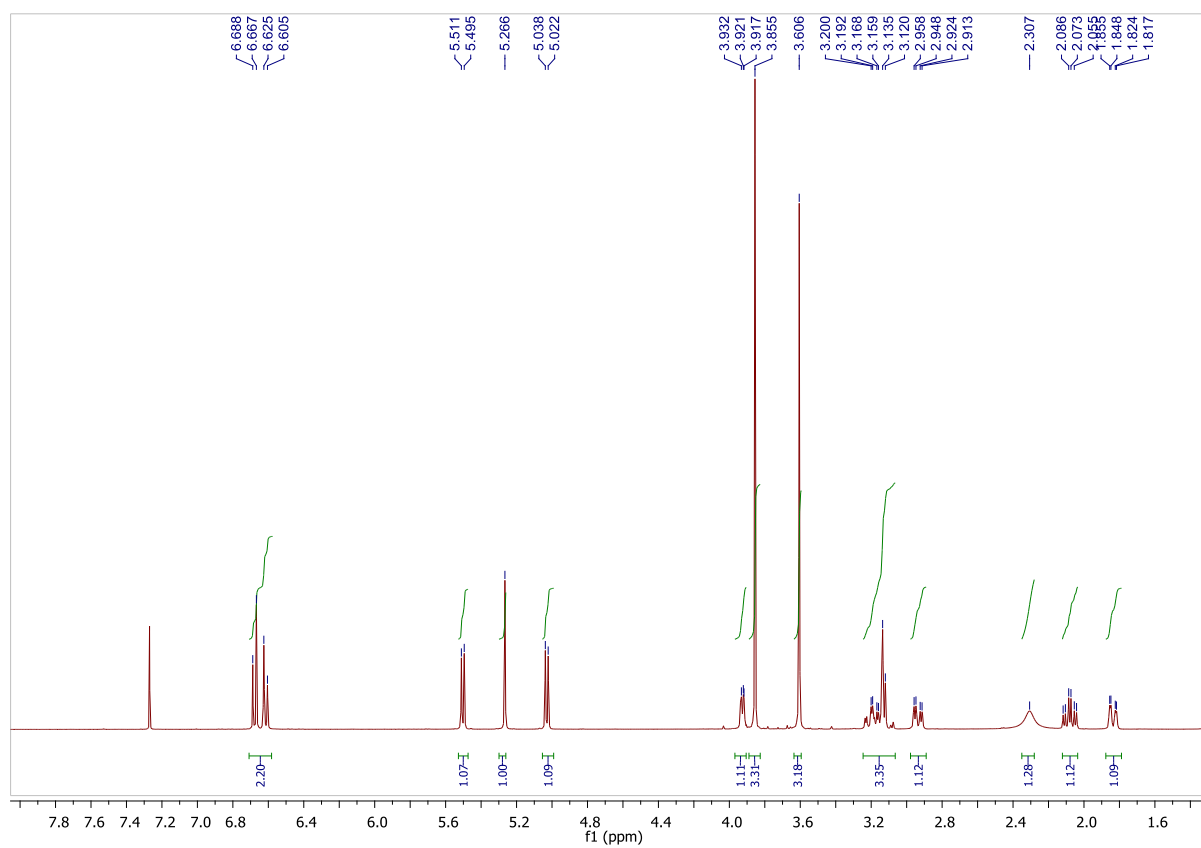
Figure 10. ^1\text{H} NMR spectrum of N -Northebaine in \text{CDCl}_3
