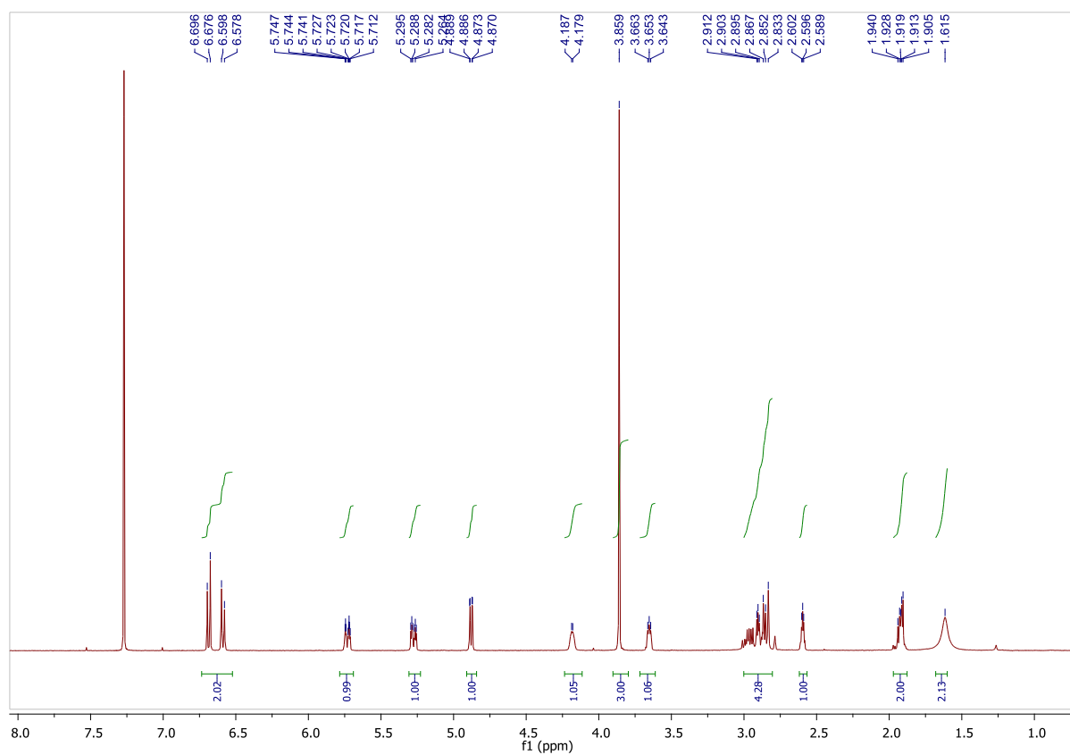
Figure 4. ^1\text{H} NMR spectrum of N -Norcodeine in \text{CDCl}_3
