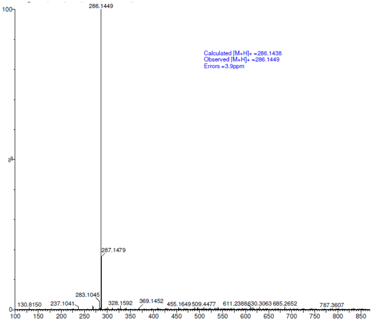
Figure 6. High Resolution MS of N -Norcodeine
