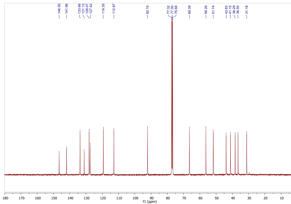
Figure 5. ^{13}\text{C} NMR spectrum of N -Norcodeine in \text{CDCl}_3
