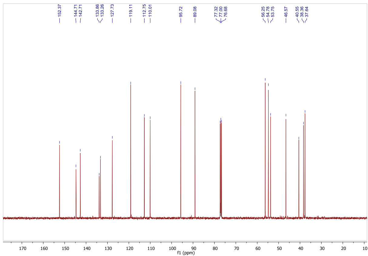
Figure 11. ^{13}\text{C} NMR spectrum of N -Northebaine in \text{CDCl}_3
