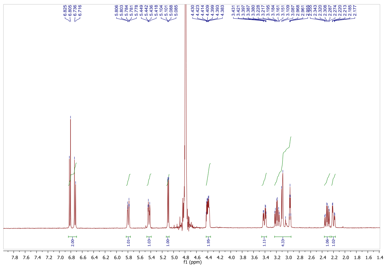
Figure 1. ^1\text{H} NMR spectrum of N -Normorphine Hydrochloride in \text{D}_2\text{O}
