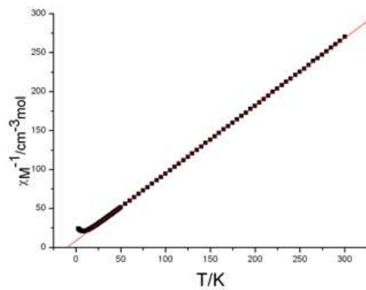
Figure S2. The exp./black and simulated/red \chi_M^{-1} versus T plots of 3 .
