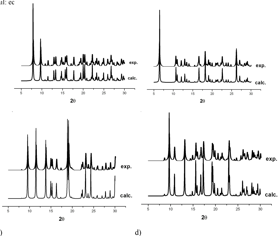
Figure S1. The experimental and simulated XRD patterns of 1-a , 2-b , 3-c , 4-d , respectively.
