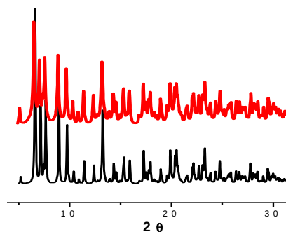
Figure S1. The experimental XRD pattern/red of bulk samples and simulated XRD pattern/black from single crystal data of 1 .
