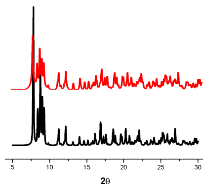
Figure S1. The experimental XRD pattern/red of bulk samples and simulated XRD pattern/black from single crystal data of 1 .
