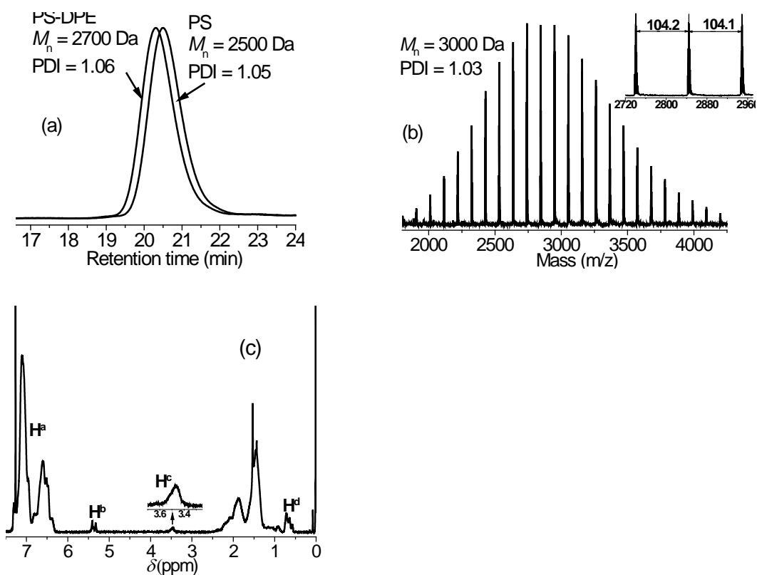
Fig. S1. GPC diagram (a), MALDI-TOF MS (b) and ^1\text{H} NMR spectrum in \text{CDCl}_3 (c) for polystyrene macromonomer, PS-DPE.
