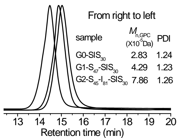
Fig. S2. GPC diagram for star-like dendrigraft copolymers and star precursor G0-SIS.
