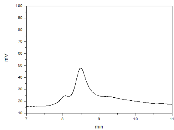
Figure S2. GPC traces of copolymer II-70%.
