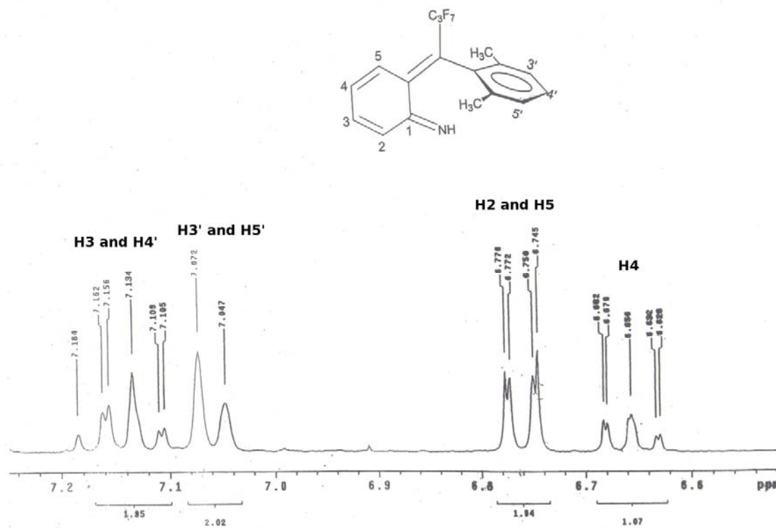
Figure S2. 1 H NMR spectrum of E-27 (300 MHz, CDCl 3 ).
