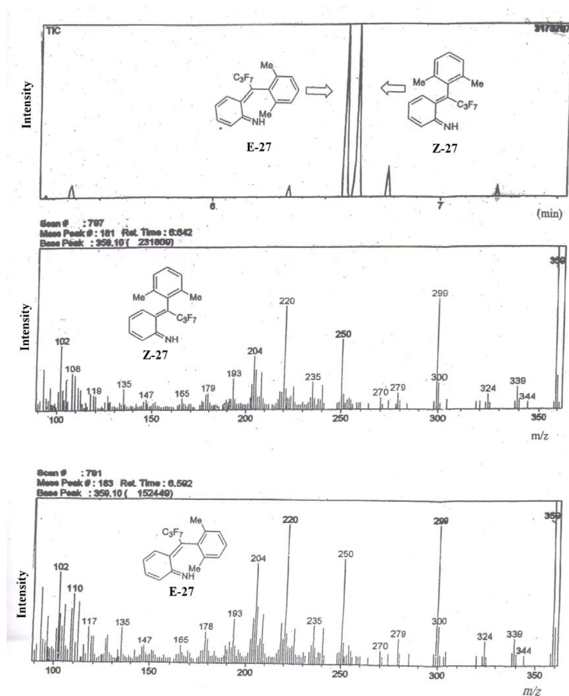
Figure S1. GC-MS analysis of intermediates products E-27 and Z-27 . The EI-mass spectra were obtained on a Shimadzu GC-17A instrument coupled to a QP-5000 mass selective detector, using a 15m0.25mm XTI-5 column coated with poly(dimethylsiloxane).
