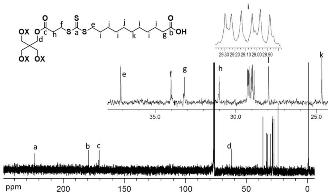
Fig.S2. ^{13}\text{C} NMR spectra (400 MHz) of tetra-functional CTA-2 with carboxylic acid end groups.
