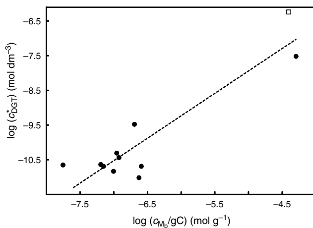
Fig. A1. Concentrations of \text{Pb}^{\text{II}} measured by DGT (diffusive gradients in thin film) in natural waters as a function of metal-to-ligand ratio in the sample. Data are shown for unspiked freshwater, pH 7 to 8 ( \bullet ) [35,41,44,59,60] and isolated humic acid (HA), pH 5.5 ( \square ). [61] d_g = 8 \times 10^{-4} m. The dashed line corresponds to the regression line used to compute \Gamma .
