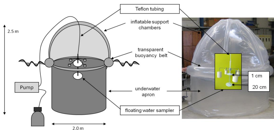
Fig. S1. Design of free floating surface mesocosm.
