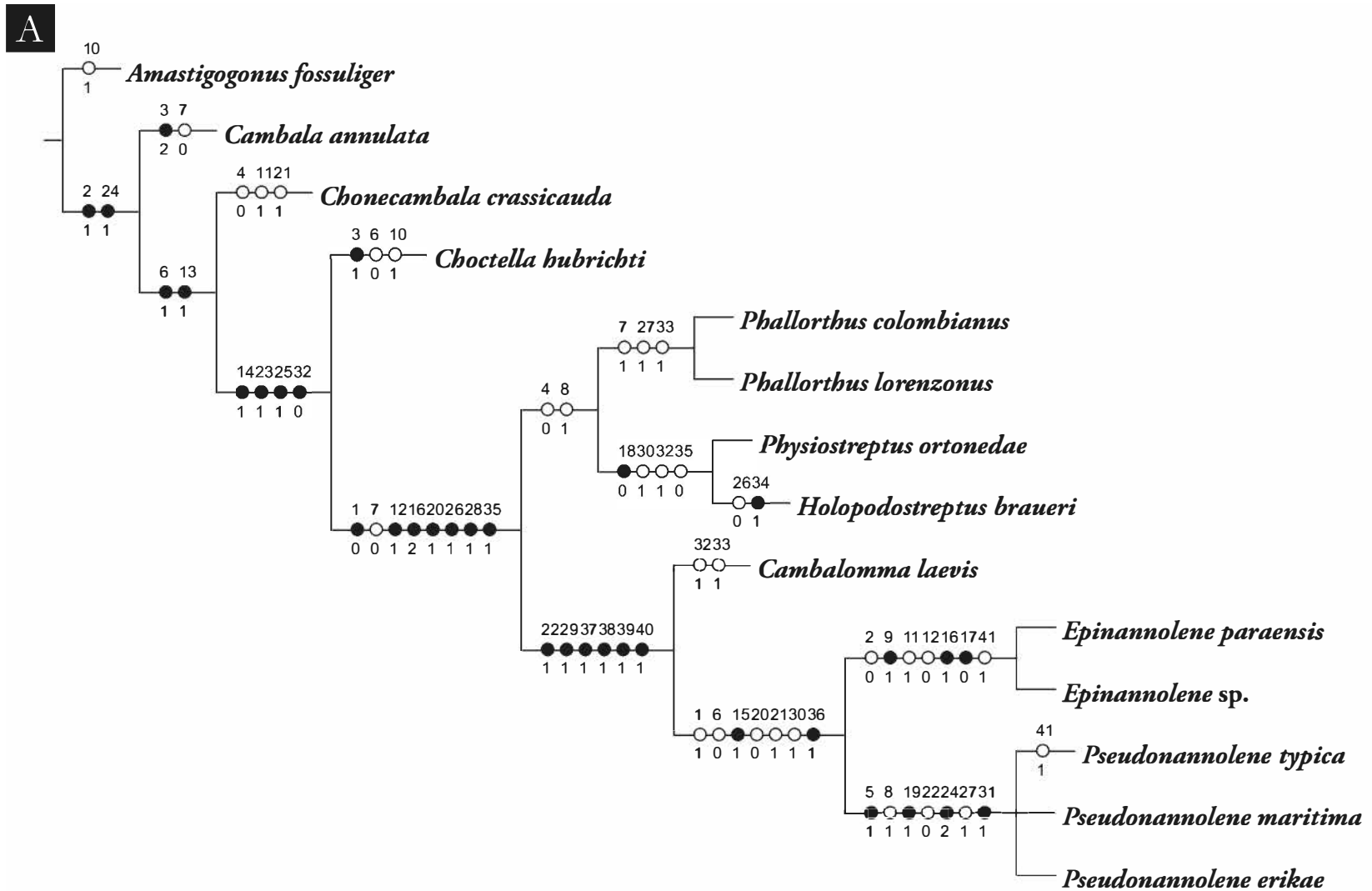
Fig. S1. The most parsimonious tree obtained with implied weighting of the characters ( k = 6 ) under AccTran optimisation (A) and DelTran optimisation (B). Black circles correspond to unique transformations, and white circles correspond to homoplastic transformations.
