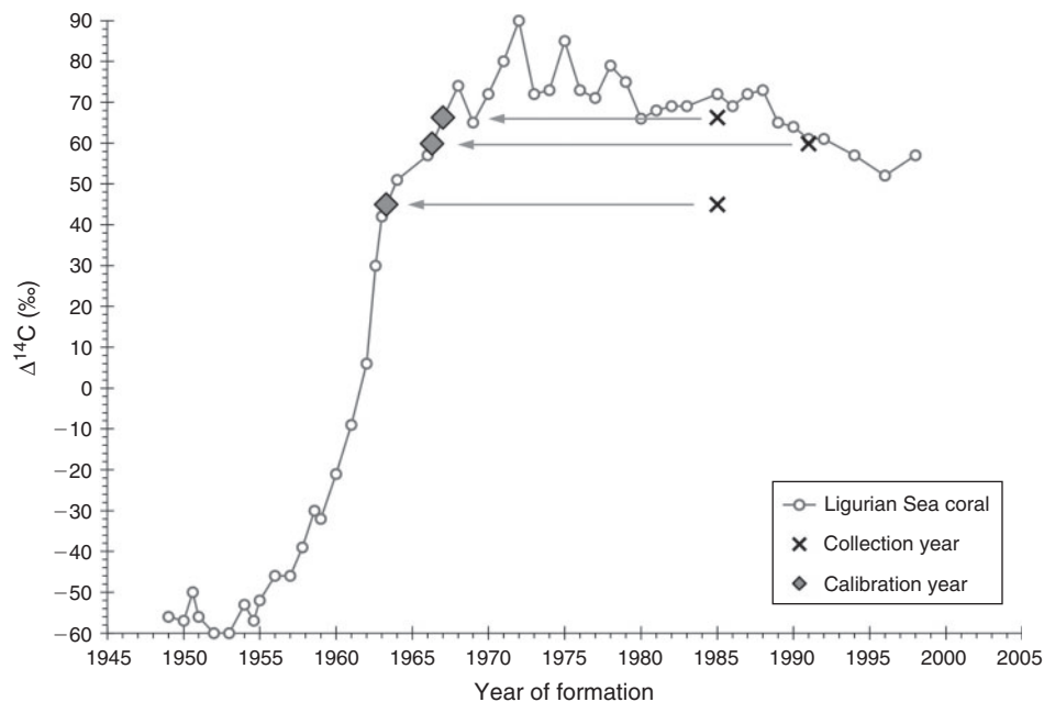
Fig. 1. Plot of the \Delta^{14}\text{C} reference series from a coral in the Ligurian Sea (Tisnérat-Laborde et al. 2013) with the measured \Delta^{14}\text{C} values from otolith cores of three of the largest adult European hake from the Mediterranean Sea. Each measured value is plotted initially at the date of collection and is then projected back in time to the \Delta^{14}\text{C} reference to determine the year of formation or validated birth year.
