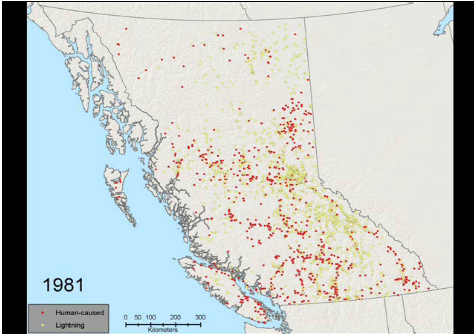
Fig. S1. Annual distribution of lightning (yellow) and person-caused (red) fires in British Columbia during 1981-2000 [Click on image to view animation].
