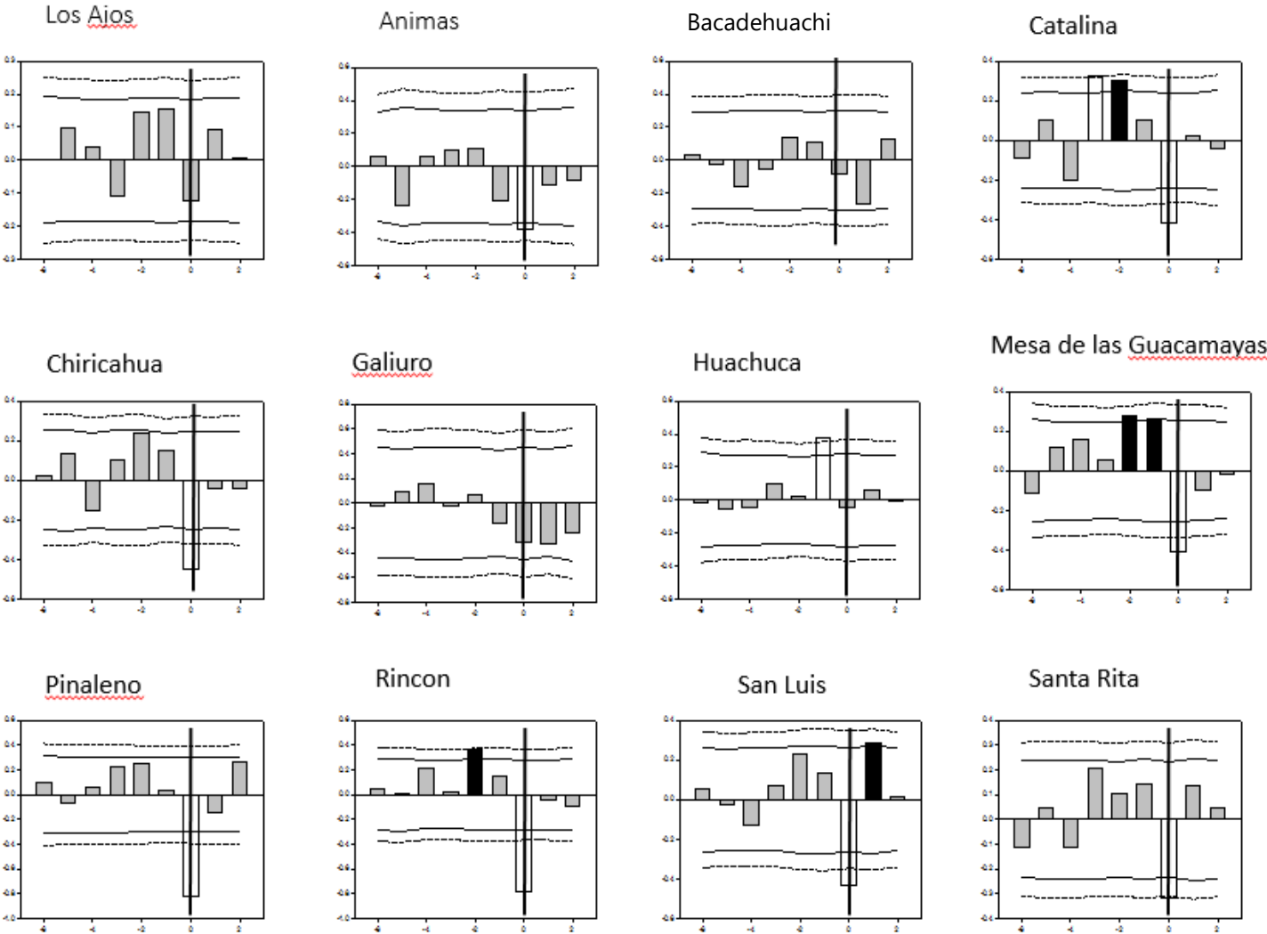
Fig. S1. Superposed Epoch Analysis based on Winter SPI for all mountain ranges in the study. Figure layout is as in Figure 4 in the main text.
