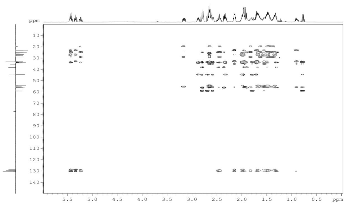
Figure S4. HSQC spectrum of acanthocyclamine A 1 in CDCl 3
