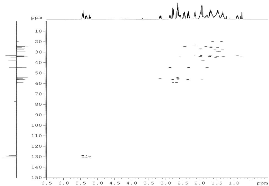
Figure S4. HSQC spectrum of acanthocyclamine A 1 in CDCl 3
