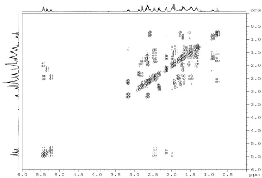
Figure S6. DQFCOSY spectrum of acanthocyclamine A 1 in CDCl 3
