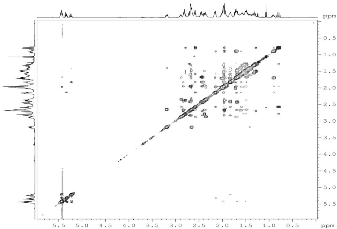
Figure S7. NOESY spectrum of acanthocyclamine A 1 in CDCl 3
