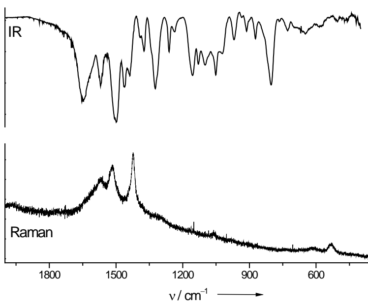
Fig. S2. Comparison between the IR and Raman spectra of [3(\text{CuCl}_2)_4] .
