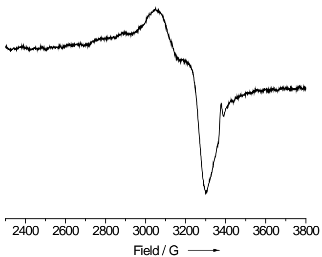
Fig. S1. EPR spectrum of [3(\text{CuCl}_2)_4] at 120 K in frozen \text{CH}_2\text{Cl}_2 .
