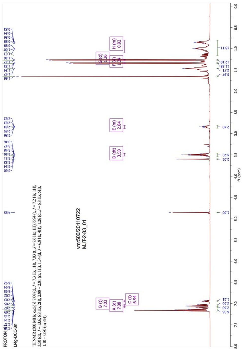
Figure S4. ^1\text{H} NMR spectrum of [(\text{BDI})\text{Mg}(\text{BnC}\{\text{NCy}\}_2)] ( 4 ).
