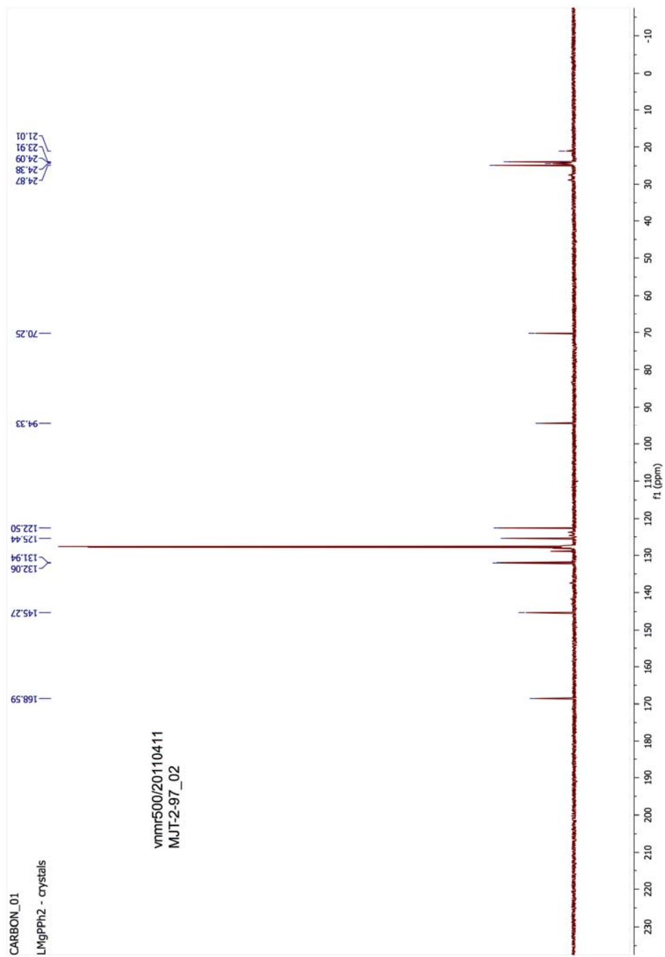
Figure S7. ^{13}\text{C} NMR spectrum of [(\text{BDI})\text{Mg}(\text{PPh}_2)(\text{THF})] ( 5 ).
