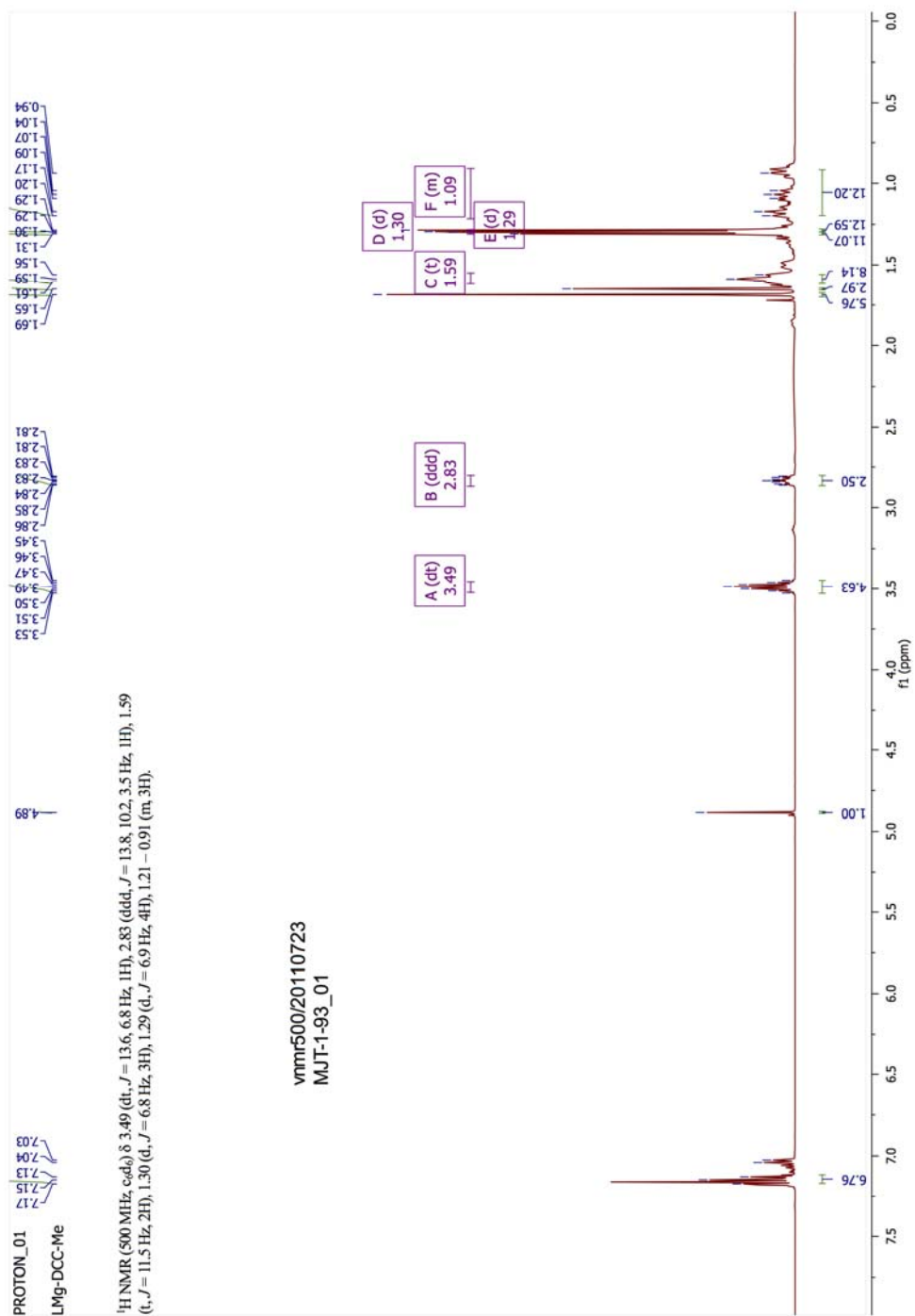
Figure S1. ^1\text{H} NMR spectrum of [(\text{BDI})\text{Mg}(\text{MeC}\{\text{NCy}\}_2)] ( 3 )
