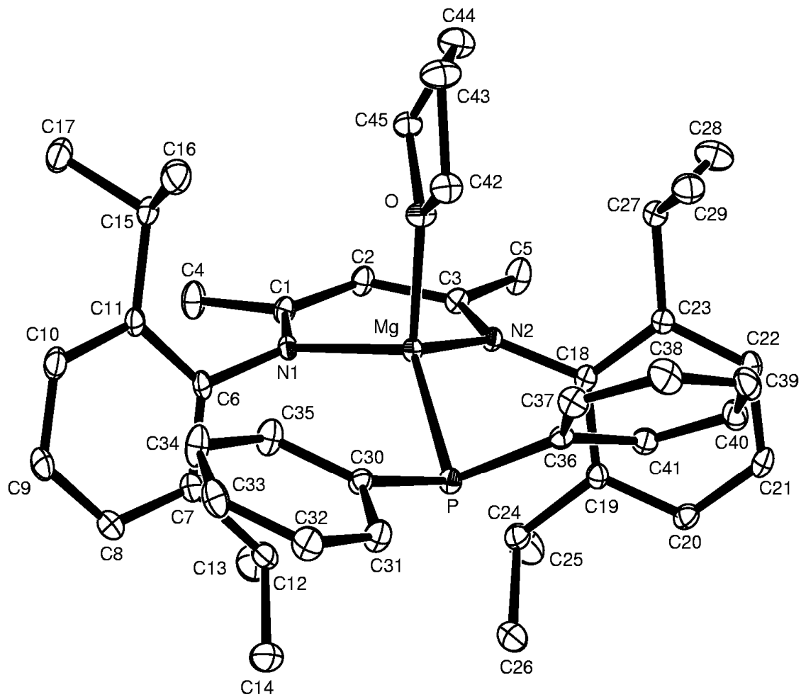
Figure S8. Thermal ellipsoid plot of [(BDI)Mg(PPh 2 )(THF)] ( 5 ).
