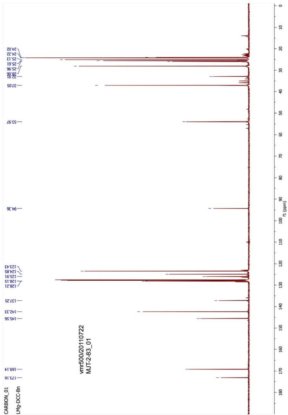
Figure S5. ^{13}\text{C} NMR spectrum of [(\text{BDI})\text{Mg}(\text{BnC}\{\text{NCy}\}_2)] ( 4 ).
