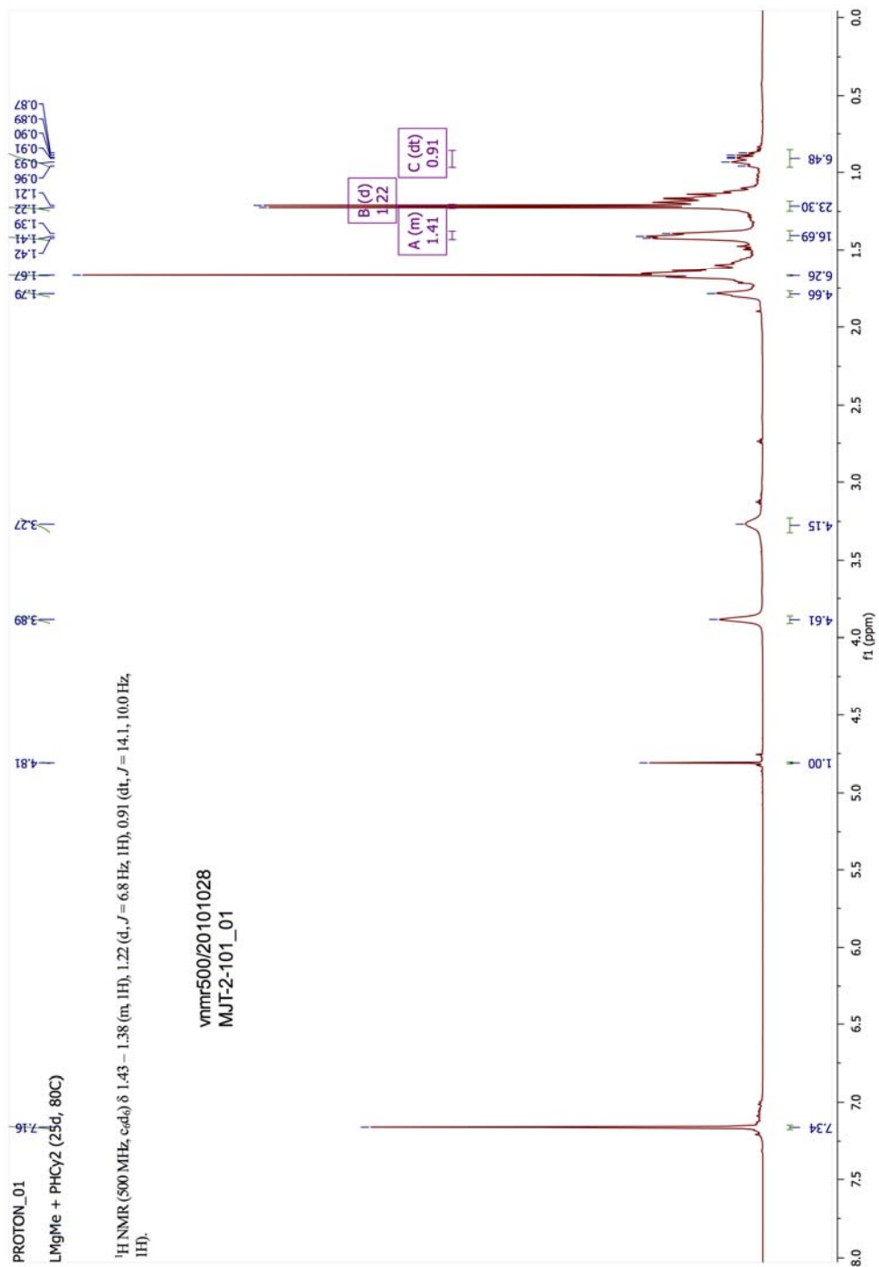
Figure S9. ^1\text{H} NMR spectrum of [(\text{BDI})\text{Mg}(\text{PCy}_2)(\text{THF})] ( 6 ).
